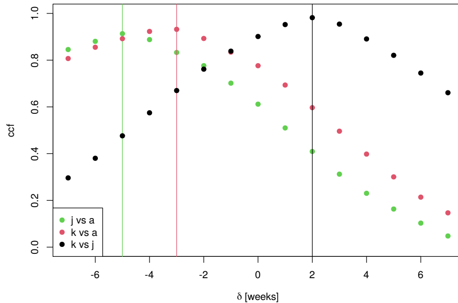
Figure 2: Cross-correlation functions by phase shift \delta for I_x(t+\delta) versus I_y(t) for the three (x, y) -pairs (j, a) , (k, a) , (k, j) , respectively, during the first two waves ( t < 60 weeks). For each pair, maximum \delta is highlighted by a vertical line.
