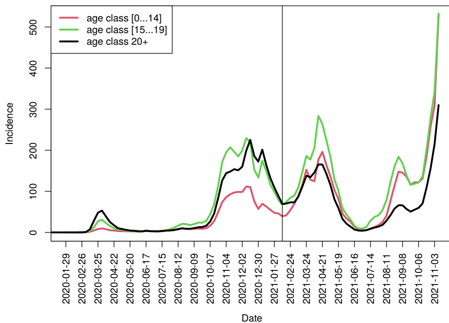
Figure 1: German-wide 7-day-incidence (per 100,000) time series for children, juveniles, and adults, respectively, sampled per week. Mutual cross-correlations are calculated for the two temporal intervals separated by the vertical line (at week 59).
