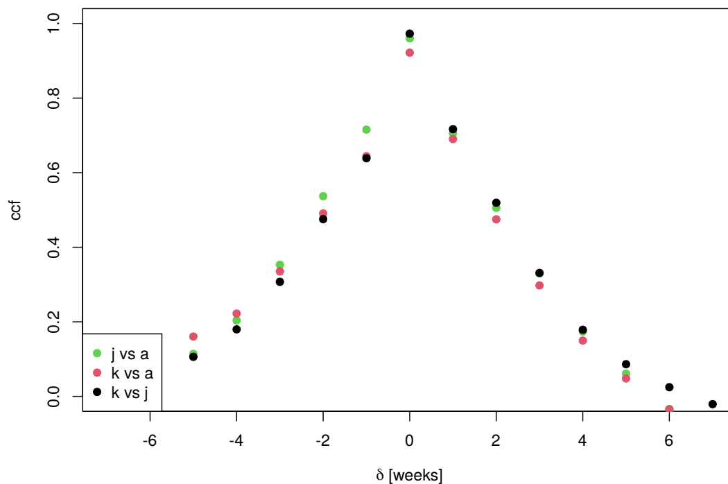
Figure 4: Cross-correlation functions by phase shift \delta for I_x(t+\delta) versus I_y(t) for the three (x, y) -pairs (j, a) , (k, a) , (k, j) , respectively, during the second half of the epidemic ( t > 59 weeks).
