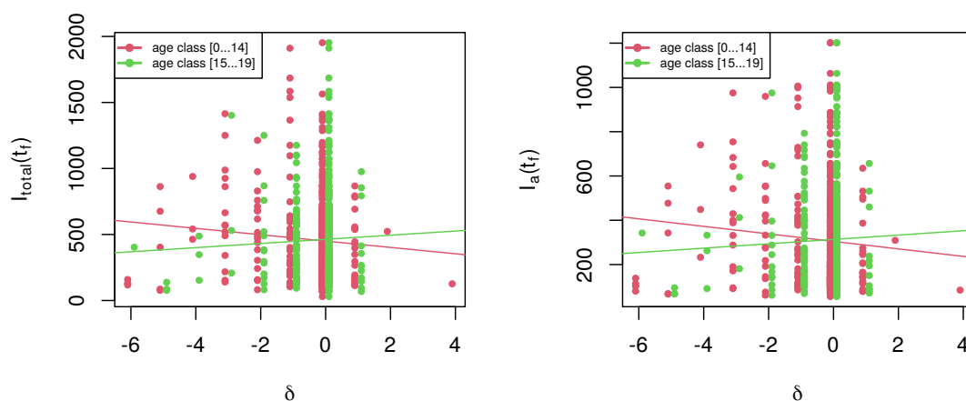
Figure 3: Linear regression predicting the current ( t_f = 17 Nov 2021) total incidence (left panel) and the incidence of the adult sub-population (right panel), respectively, observed in the 411 German districts by the phase shift between I_j(t) and I_a(t) (green) or alternatively by the phase shift between I_k(t) and I_a(t) (red) for t < 60 weeks.
