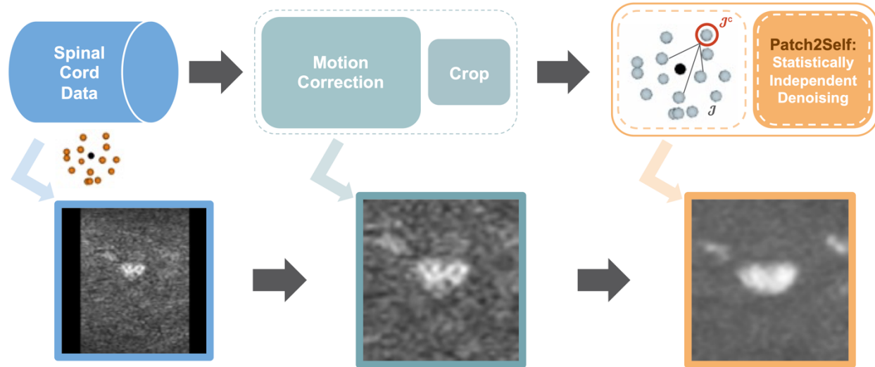
Figure 2. Image processing pipeline. Diffusion data were motion corrected using the Spinal Cord Toolbox, then Patch2Self (implemented in DIPY) was applied to cropped, motion-corrected volumes.
