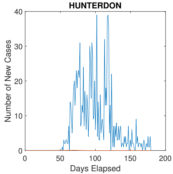
Figure 4: The genetic algorithm (red) has not optimized the residual for Hunterdon County well because it has very few cases (at max 40 per day). Also note the importance of smoothing the data to remove outliers with 0 cases.
