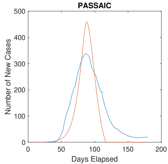
Figure 3: Graph (red) overlaid on collected data (blue) for Passaic County, NJ (Specify the final genetic information used for the result.)
