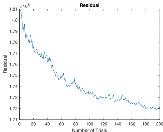
Figure 1: The residual of the SIR Model getting lower as the genetic algorithm optimizes the variables to better fit the collected data.
