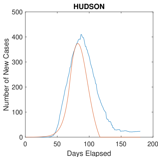
Figure 2: The SIR Model created curve (red) overlaid on top of recorded new cases (blue) for Hudson County, NJ
