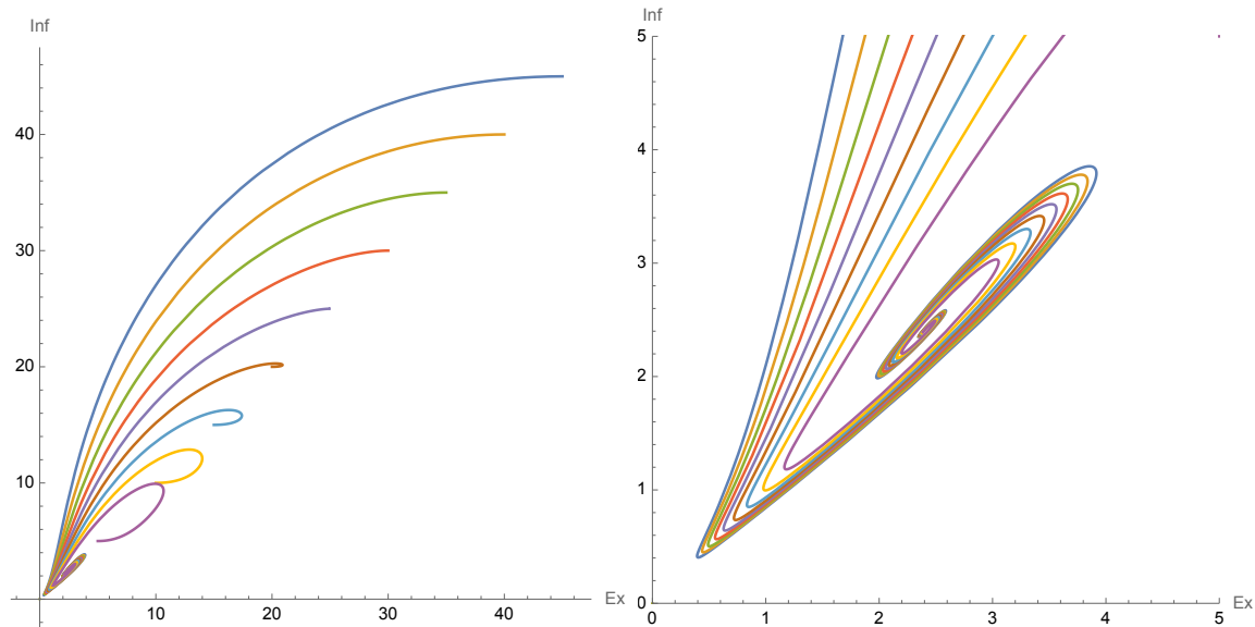
FIGURE 2. The endemic equilibrium of Example 2.5 with colors as in Figure 1. The left plot displays the I versus E compartments. The right plot shows the same, zooming in on the equilibrium point.
