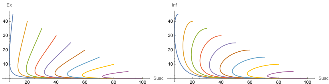
FIGURE 3. The disease-free equilibrium of Example 2.8. Plots as in Figure 1.
