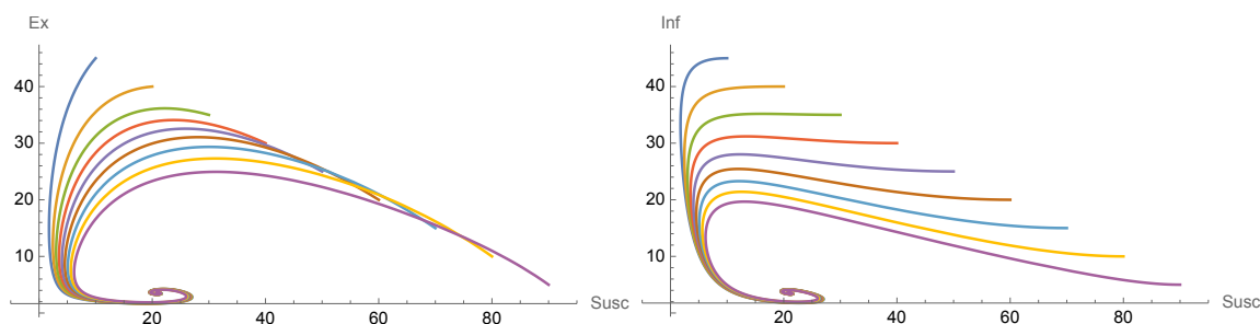
FIGURE 4. The endemic equilibrium of Example 3.3. Plots as in Figure 1.
