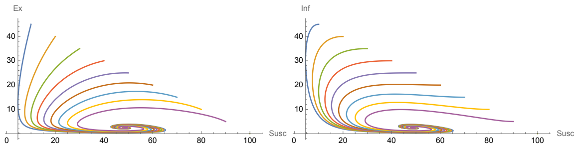
FIGURE 1. The endemic equilibrium of Example 2.5. The left plot displays E versus S compartments, while the right plot displays I versus S compartments. Each colored curve represents a different initial condition of the form (S, E, I, R) = (S_0, (n - S_0)/2, (n - S_0)/2, 0) for S_0 = 10, 20, \dots, 90 .
