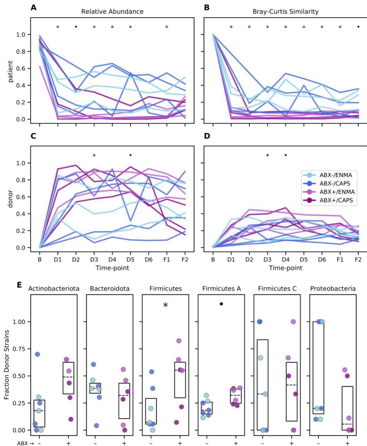
Figure 3: Greater community perturbation and engraftment of donor strains following FMT treatment in antibiotic-pretreated patients. (A, C) Abundance of strains specific to each patient's baseline sample (A) or specific to each donor sample (C) relative to the patient's total strain populations over the course of treatment. (B, D) BC similarity (1 - BC dissimilarity) between each patient's sample and that patient's own
