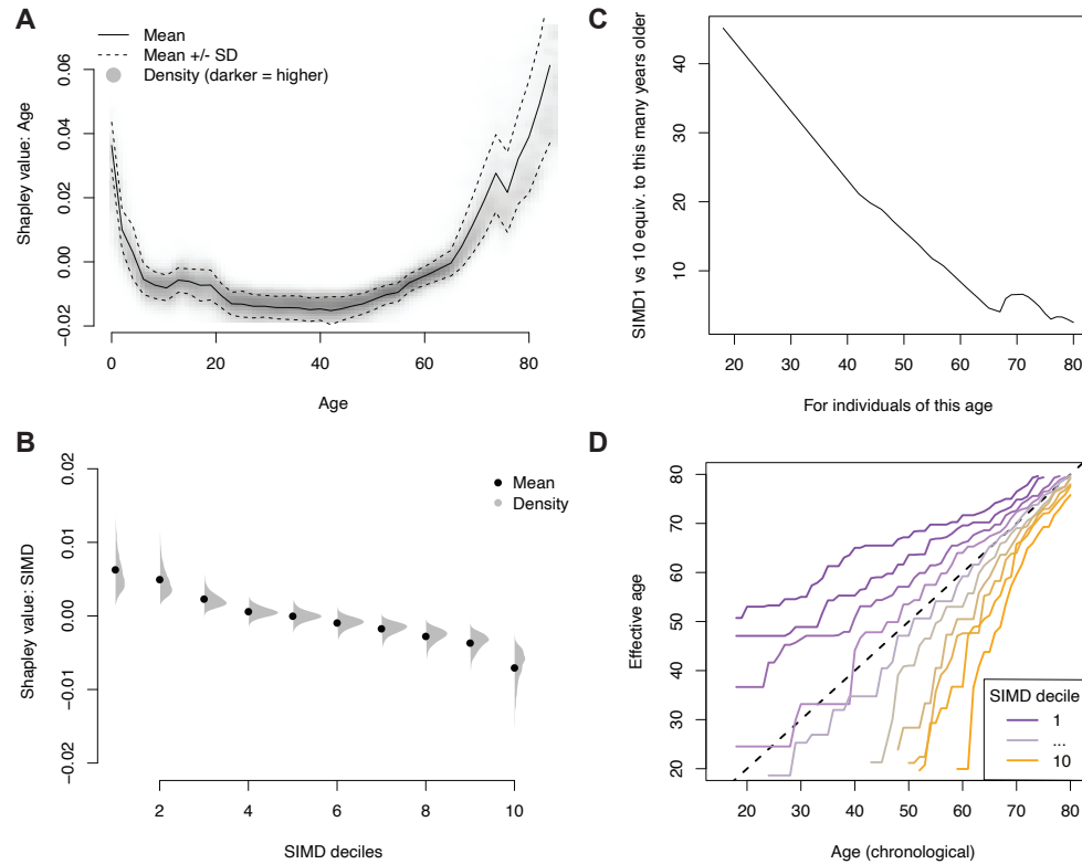
Figure 5: Analysis of Shapley values. Distribution of Shapley values by (A) age and (B) SIMD deciles (1: most deprived; 10: least deprived). (C) Number of additional years of age needed to match the difference in Shapley values between SIMD deciles 1 and 10. (D) 'Effective ages' calculated to match EA rates: for an (age, SIMD decile) pair, the age at mean SIMD with the equivalent EA rate.
