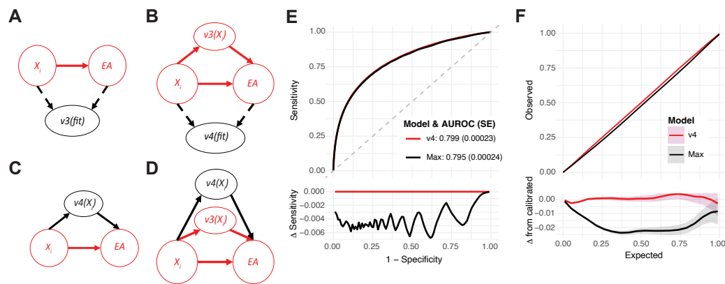
Figure 6: Model updating in the presence of performative effects. (A-D) Causal structure for the training and deployment of SPARRAv3 and SPARRAv4. X_i represents covariates for a patient-time pair; v3(\text{fit})/v4(\text{fit}) and v3(X_i)/v4(X_i) represent the fitting and deployment of v3 and v4 respectively. (A) Training setting for SPARRAv3. (B) Training setting for SPARRAv4. (C) Deployment setting if SPARRAv4 were to naively replace SPARRAv3. (D) Deployment setting in which SPARRAv4 is used as an adjuvant to SPARRAv3. (E) Comparison of discrimination (ROC) between SPARRAv4 and the maximum of both scores. (F) Comparison of calibration between SPARRAv4 and the maximum of both scores.
