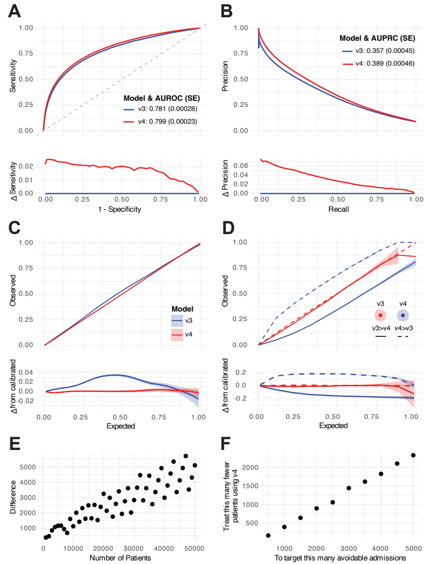
Figure 2: Comparison of overall predictive performance between SPARRA v3 and SPARRA v4. (A) ROC. (B) PRC. Lower sub-panels show differences in sensitivity and precision, respectively. Confidence intervals are negligible. (C) Calibration curves. (D) Calibration curves for samples in which |v4 - v3| > 0.1 . Lower sub-panels show the difference between curves and the y = x line (perfect calibration). Confidence envelopes are pointwise (that is, for each x -value, not the whole curve). Predicted/true value pairs are combined across cross-validation folds in all panels for simplicity. (E) Difference in the number of individuals who had an event amongst individuals designated highest-risk by v3 and v4. The repeating pattern is a rounding effect of v3. (F) Difference in the number of highest-risk individuals to target to avoid a given number of admissions.
