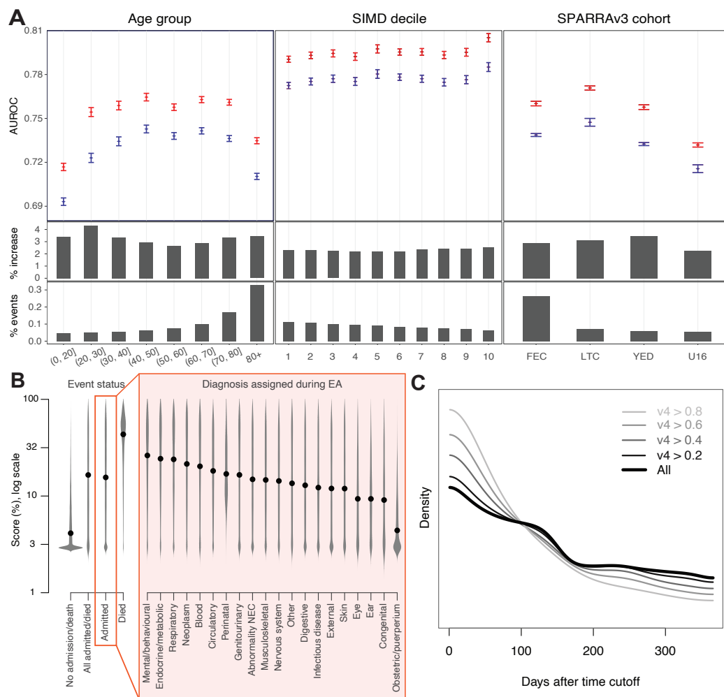
Figure 3: Stratified performance of SPARRAv3 and SPARRAv4. (A) Performance of SPARRAv3 and SPARRAv4 in subcohorts defined by age, SIMD and the original subcohorts defined during SPARRAv3 development (Methods). Top: AUROC (blue: SPARRAv3; red: SPARRAv4). Vertical bars denote plus/minus 3 standard deviations. Middle: AUROC increase for SPARRAv4 with respect to SPARRAv3. For context, bottom sub-panels show the proportion of samples with an event within each group. (B) Distribution of SPARRAv4 scores (in log-scale) based on the type of diagnosis recorded during the admission (see Supplementary Table S5 for definitions). Black points indicate the associated medians. Groups were defined according to whether an event was observed (grey violin plots) or, for those with an EA, based on the diagnosis recorded during the admission (black violin plots). (C) Density of time-to-first-EA (that is, days between time cutoff and first EA date) in subsets of individuals who had an EA in the year following the time cutoff and had a SPARRAv4 score above a given cutoff. For instance, the lightest line shows density of time-to-first-EA in samples who had an EA and had SPARRAv4 4 0.8
