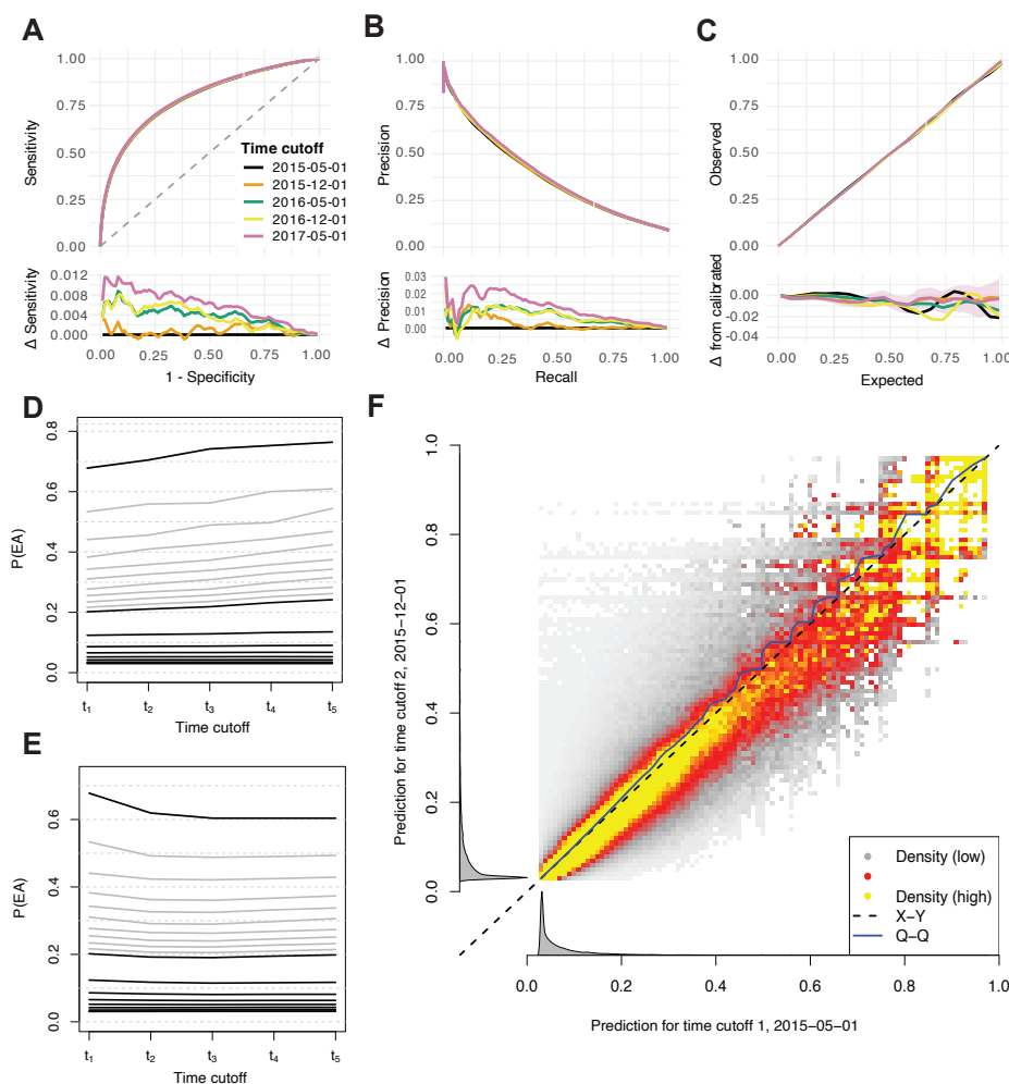
Figure 4: Performance of a static model with changing scores over time. (A-C) Performance of scores calculated at t_1 - t_5 from static model M_0 . (A) ROC curves. Lower panel shows differences in sensitivity with respect to t_1 . (B) PRC curves. Lower panel shows differences in precision with respect to t_1 . (C) Calibration curves. Lower panel shows the difference between observed and expected EA frequency. (D) Centiles (grey) and deciles (black) of risk scores (calculated using M_0 ) over time, across all individuals with data available at all time cutoffs. (E) Average score over time for groups of individuals defined by risk centiles (grey) and deciles (black) at time t_0 (2 May 2015). (F) Density (low to high: white-grey-red-yellow) of scores generated using the static model M_0 to predict EA risk at t_1 (2 May 2015) and t_2 (1 Dec 2015). The density is normalised to uniform marginal on the Y axis, then the X axis; true marginal distributions of risk scores are shown alongside in grey.
