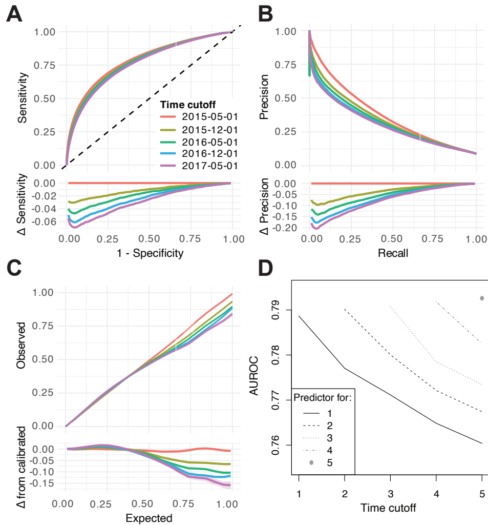
Figure S4. Performance of a static model and static scores used to predict risk at future time cutoffs. (A-C) Performance of static scores evaluated using M_0 at time t_0 for predicting EA at times t_1 - t_5 . (A) ROC curves. (B) PR curves. (C) Calibration curves. (D) AUROCs for scores calculated at each time cutoff (based on M_0 ) for prediction in subsequent time cutoffs.
