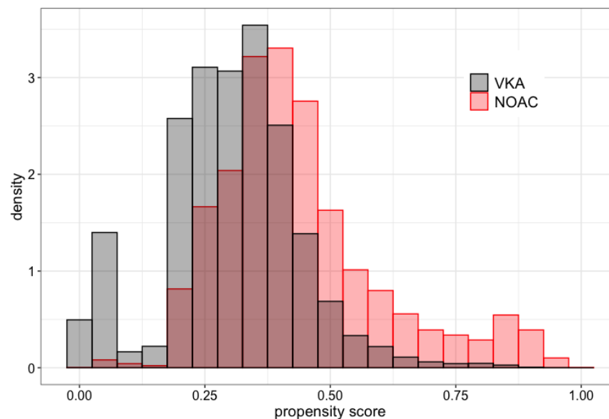
Figure 2: Propensity score at the start of follow-up
