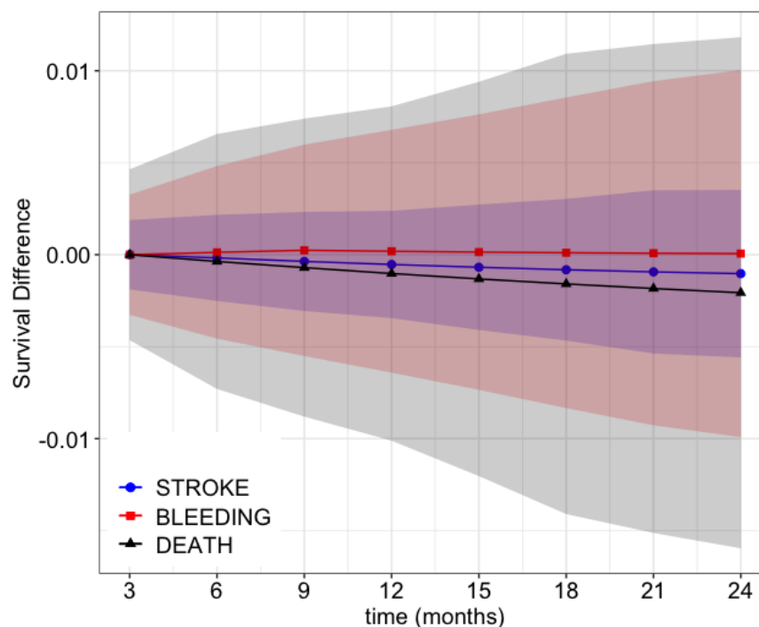
Figure 3: Estimated average treatment effect (ATE) for selected outcomes using TMLE adjusted potential outcomes from a SuperLearner model. The solid line corresponds to the average and the shaded areas correspond to the 95% confidence intervals.
