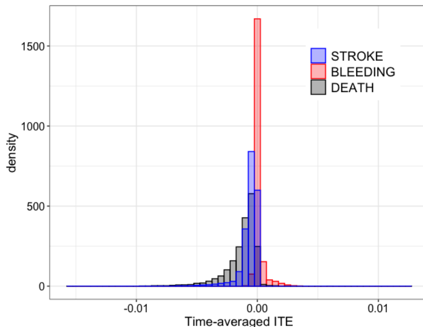
Figure 4: Distribution of time-averaged individual treatment effects (ITE) for selected outcomes using a SuperLearner model
