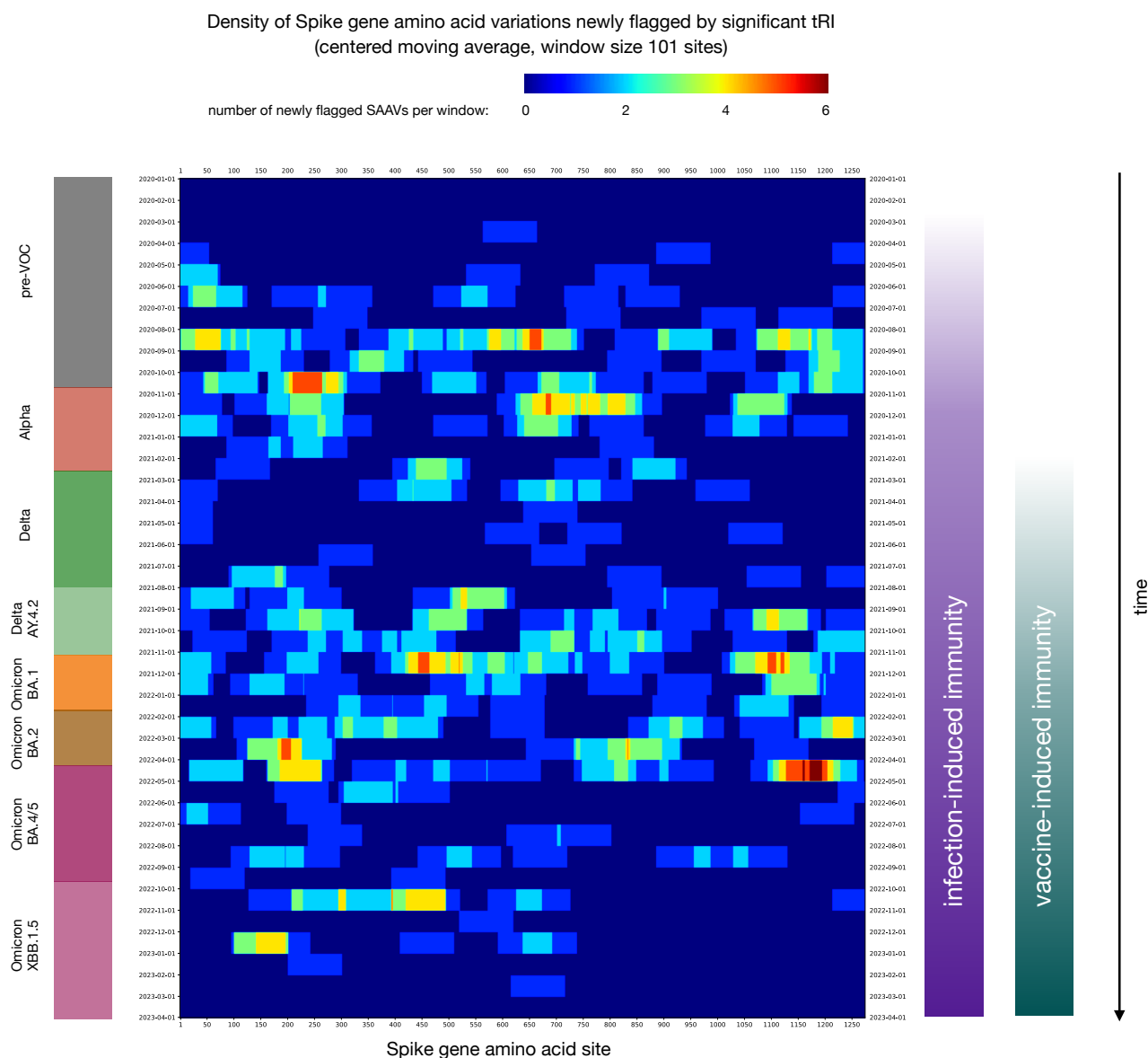
Figure 7. Topological recurrence and the SARS-CoV-2 fitness landscape. Dynamics of the interaction between topological signals of recurrence and host immunity/waves of dominant variants in the United Kingdom. For each month from January 2020 until March 2023, the heatmap shows the density of Spike gene amino acid variations for which the topological signal (tRI) turned significant during that month (density is centered moving average with window size of 101 sites). Topological recurrence analysis based on GISAID data from the UK covering the whole pandemic from December 2019 until March 2023 (see Methods ); additional epidemiological information taken from Carabelli et al. [77, Figure 4].
