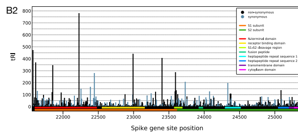
Figure 4. Topological signals during the first year of the pandemic. Topological recurrence analysis for the whole genome and the Spike gene from December 2019 until February 2021. The tables in (A1) and (B1) list the topological recurrence index (tRI) and the prevalence for mutations with strongest topological signal. In each table the last column reports filtration rules recommended in Turakhia et al. [33, 46] and De Maio et al. [47] for highly homoplastic sites, problematic sites and potential artifacts that are normally removed or masked in SARS-CoV-2 phylogenetic analyses. For a complete list see Supplementary Information Table 1 and Supplementary Information Table 2 . (A2) Histogram showing the distribution of topological signals across the whole genome. In every region of the genome, reticulate events play a crucial role in the evolution of the virus. (B2) Histogram showing the distribution of topological signals across the Spike gene. There is an accumulation of topologically recurrent mutations in the S1 subunit and the S1-S2 cleavage region, as well as in the signal peptide at the beginning of the Spike gene.
