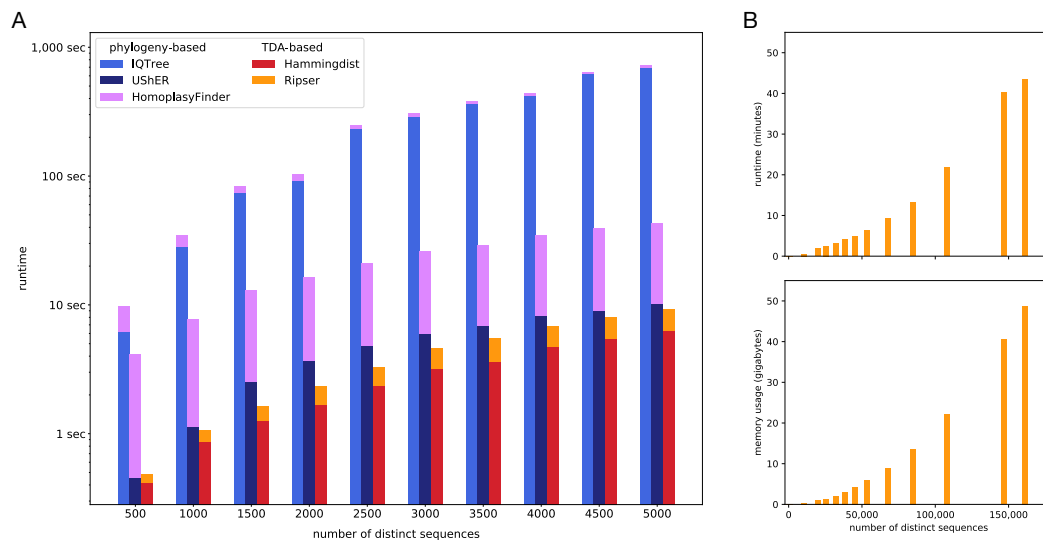
Figure 3. Performance analysis and comparison with phylogeny-based methods. (A) Basic runtime comparison between Topological Data Analysis (TDA)-based methods and phylogeny-based methods for random samples of up to 5,000 SARS-CoV-2 genomes. We used IQTree [35] and UShER [29] to reconstruct phylogenetic trees. The subsequent homoplasy analysis was performed with HomoplasyFinder [9]. For the TDA-approach we used Hammingdist [41] to generate genetic distance matrices and Ripser [40] for the subsequent computation of persistence barcodes (see Methods ). (B) Runtime and memory usage for the computation of persistence barcodes with Ripser [40] for monthly sub-alignments of the GISAID alignment with 161,024 genetically distinct whole genome sequences covering the first year of the pandemic (see Methods ).
