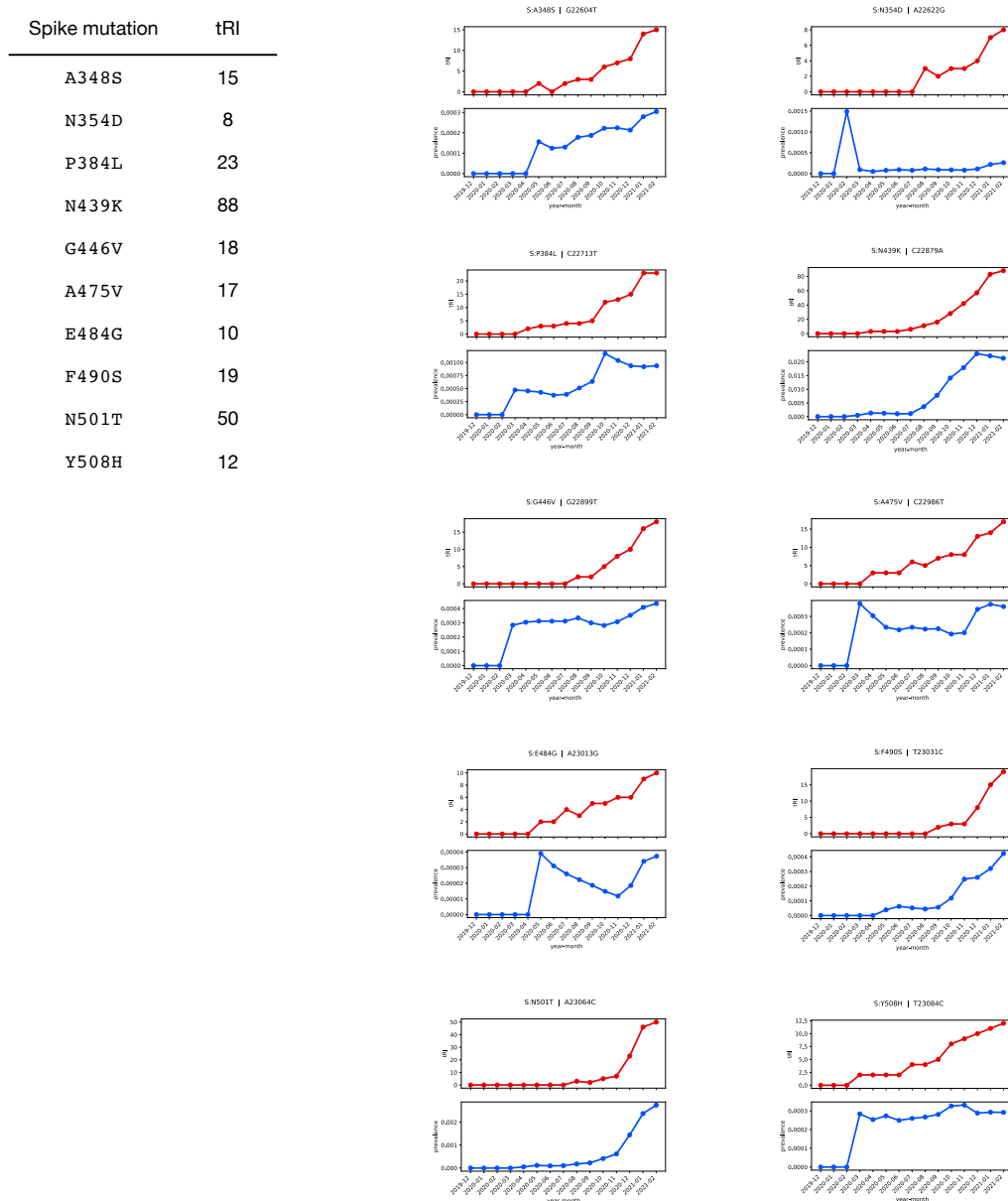
Supplementary Information Figure 4. Surveillance of emerging escape mutations on the receptor-binding domain. Comparative time series analysis charts (tRI vs. prevalence) for mutations on the receptor-binding domain that showed a significant tRI signal with rising tendency in February 2021 and are associated with an increased mean plasma antibody escape > 0.01 [4]. These mutations had low prevalence < 5\% and were not seen in any VOI/VOC as of February 2021 (see Supplementary Information Figure 2 ), but mutations at corresponding residues are likely to confer a fitness advantage to the virus and might therefore appear in future variants. In fact, the immune escape mutations S:G446S [4, 84] and S:F490S [4, 80] later appeared in the Lambda [85, 86] and Omicron [87] variants, which were designated as VOI/VOC in June/November 2021 [71].
