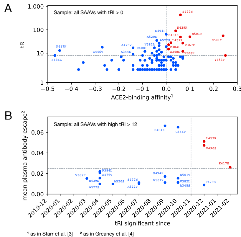
Figure 6. Topological recurrence and SARS-CoV-2 phenotypic variation during the first year of the pandemic. Both diagrams visualize contingency tables underlying Fisher’s exact test. (A) There is a strong correlation between a significant topological recurrence index ( tRI \geq 8 ) and an increase in ACE2-binding affinity in the year from December 2019 until February 2021. (B) Among highly topologically recurrent amino acid changes ( tRI > 12 ), more recent ones show increased mean plasma antibody escape. There is a significant correlation between increased mean plasma antibody escape > 0.025 and the initial acquisition of a significant tRI signal after October 2020 (Fisher’s exact test, p < 0.05 ). Experimental data taken from Starr et al. [3, Table S2] and Greaney et al. [4, Table S3].
