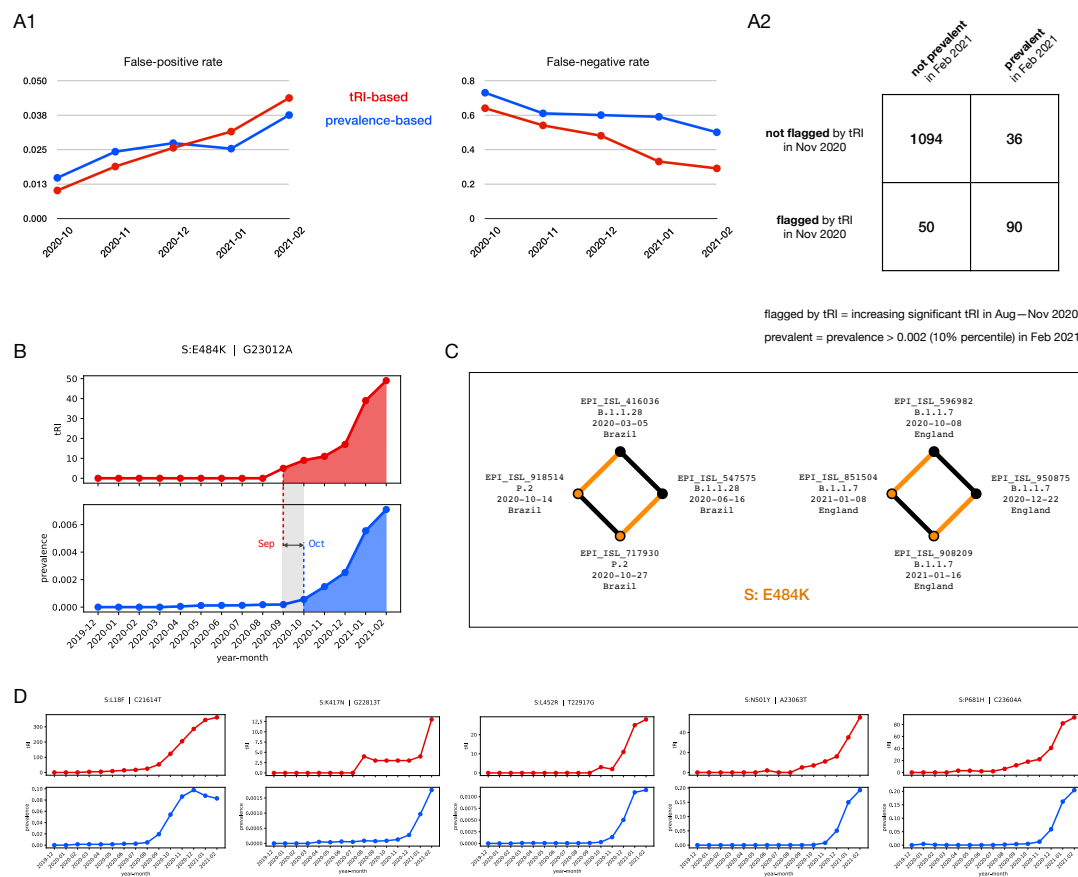
Figure 8. Surveillance of emerging potentially adaptive Spike gene mutations. (A) Specificity and sensitivity of tRI-based vs. prevalence-based identification of variable Spike amino acid sites likely to become highly prevalent (prevalence contained in 10% percentile of all mutations) three months thereafter. (A1) Reliability of identifications for each of the months October 2020 through February 2021. While false-positive rates of tRI-based and prevalence-based analyses are similar and remain small, the false-negative rates of tRI-based analyses is better than that of prevalence-based analyses (29% vs. 50%). (A2) Contingency table for tRI-based analyses for February 2021. Variable Spike amino acid sites were flagged if they exhibited a significant and increasing tRI signal from August until November 2020, and designated prevalent if their prevalence was contained in the 10% percentile of all mutations in February 2021. (B) Typical comparative time series pattern (tRI vs. prevalence) of an emerging adaptive mutation as observed in the escape mutation S:E484K. The tRI rises to a significant level (tRI = 5) in September 2020, while the prevalence stays very low < 0.02% and shows a visible increase to 0.06% by a factor of 3 for the first time several weeks later in October 2020. Both tRI and prevalence show a rising tendency in February 2021. (C) Cycle localization in the genome alignment yields geographic and temporal information about the independent acquisition of S:E484K. The diagram shows SNV cycles created by reticulate events involving the Zeta variant (P.2) in Brazil in October 2020, and within the Alpha variant (B.1.1.7) in England in January 2021. (D) Typical comparative time series pattern observed in emerging adaptive Spike mutations, with the onset of significant tRI signals preceding the rise in prevalence by several weeks.
