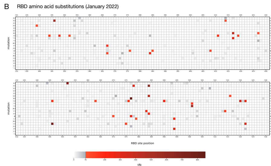
Figure 9. Topological signals for Spike gene mutations as of January 2022 and the Omicron variant. (A) The table displays selected amino acid substitutions on the Spike gene with significant topological recurrence index ( tRI \geq 76 ). For the full table see Supplementary Information Table 4 . (B) Heatmap of all amino acid variations across the RBD showing topological signals of convergence. Significant signals ( tRI \geq 76 ; shown in red) accumulate in the receptor-binding motif. (C) Topological signals of convergence for the defining Spike mutations in the Omicron variant (B.1.1.529; BA.1, BA.2 and BA.3 [88, 90, 91]). 38% of these mutations are significantly topologically recurrent with tRI \geq 76 (highlighted in boldface) and are likely due to convergent evolution. Corresponding tRI time series analysis charts are provided in Supplementary Information Figure 13 .
