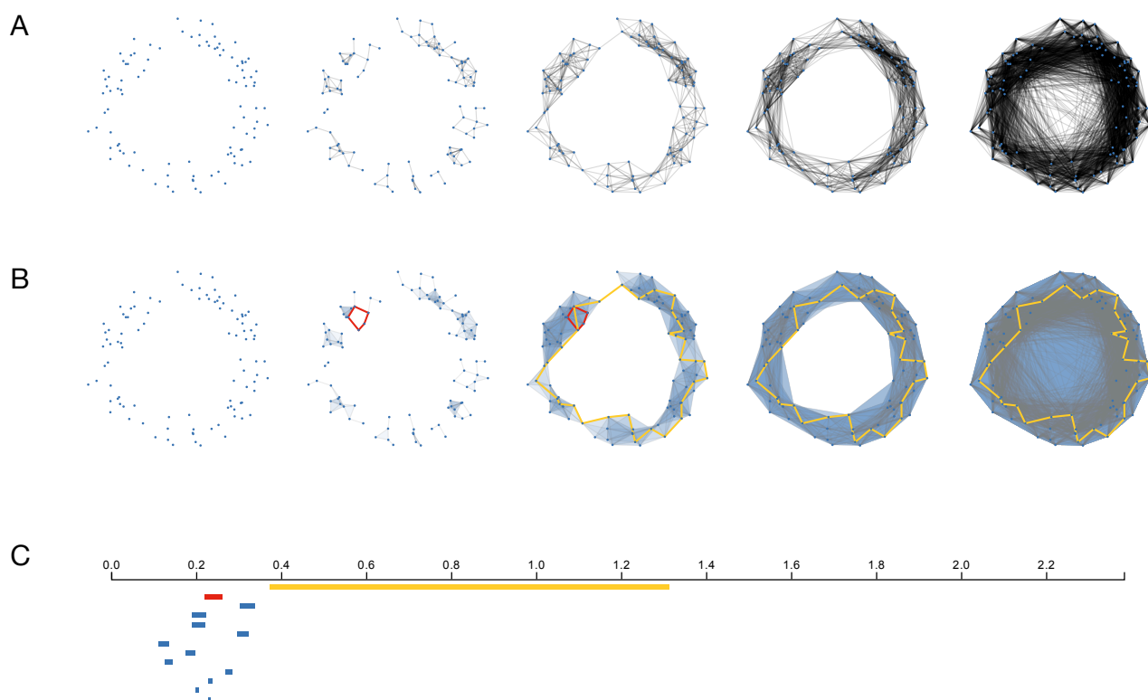
Supplementary Information Figure 8. Vietoris-Rips filtration of a point cloud. Each point represents a sample, and we display the geometric graphs (A), the resulting Vietoris-Rips complexes at different scales (B) and the persistence barcode in dimension one (C). If one only chooses one scale, one might either see nothing, or detect the small red cycle but miss the large yellow one, or vice versa. A solution to handle this issue is to characterize each cycle with its scale of appearance and disappearance: the red cycle induces a red bar in the barcode, and similarly for the yellow cycle.
