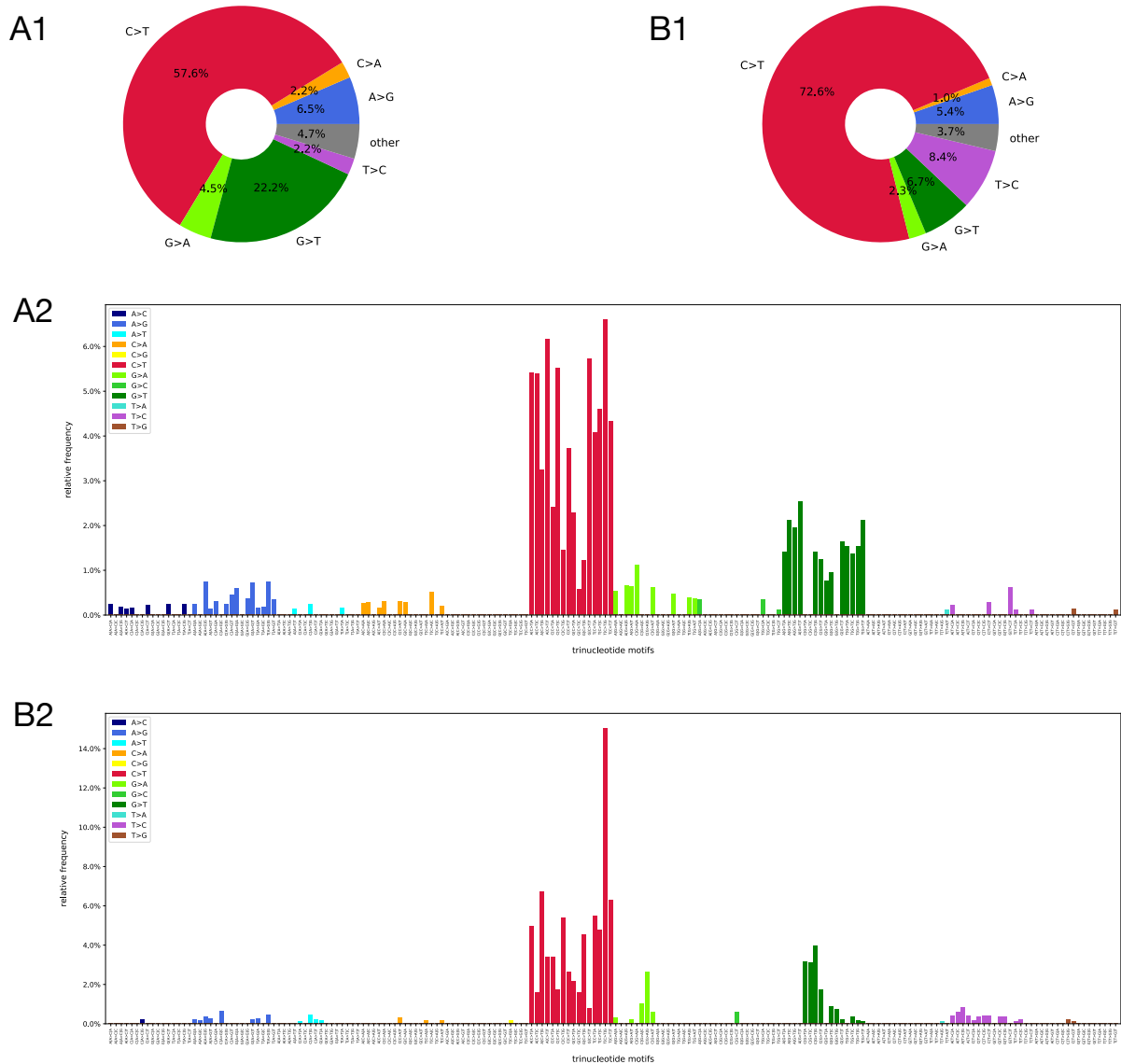
Supplementary Information Figure 7. Mutational patterns in topological signals of recurrence. Frequency analysis of nucleotide substitutions across the whole genome showing significant topological signal during the first year of the pandemic (December 2019 until February 2021). The panels display total frequencies of single nucleotide variations for non-synonymous mutations (A1) and synonymous mutations (B1). There is an excess in C-to-T transitions which suggests that the topological recurrence index also captures the action of APOBEC-mediated host RNA editing processes. Relative frequencies of trinucleotide motifs centered at single nucleotide variations for non-synonymous variations (A2) and synonymous variations (B2) (see Methods ). Statistical analyses based on Supplementary Information Table 1 .
