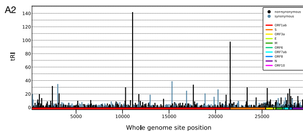
Figure 4. Topological signals during the first year of the pandemic. Topological recurrence analysis for the whole genome and the Spike gene from December 2019 until February 2021. The tables in (A1) and (B1) list the topological recurrence index (tRI) and the prevalence for mutations with strongest topological signal. In each table the last column reports filtration rules recommended in Turakhia et al. [33, 46] and De Maio et al. [47] for highly homoplastic sites, problematic sites and potential artifacts that are normally removed or masked in SARS-CoV-2 phylogenetic analyses. For a complete list see Supplementary Information Table 1 and Supplementary Information Table 2 . (A2) Histogram showing the distribution of topological signals across the whole genome. In every region of the genome, reticulate events play a crucial role in the evolution of the virus. (B2) Histogram showing the distribution of topological signals across the Spike gene. There is an accumulation of topologically recurrent mutations in the S1 subunit and the S1-S2 cleavage region, as well as in the signal peptide at the beginning of the Spike gene.
