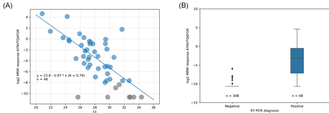
Figure 3. LC-MS (log 2 quantifier response) vs. RT-PCR (Ct) read-out correlation with linear regression (A) and quartiles distribution of the LC-MS results (B) . Color labeling is based on RT-PCR diagnoses; blue = positive SARS-CoV-2; grey = not detected (no light signals) or inconclusively quantified (single transition) by LC-MS.
