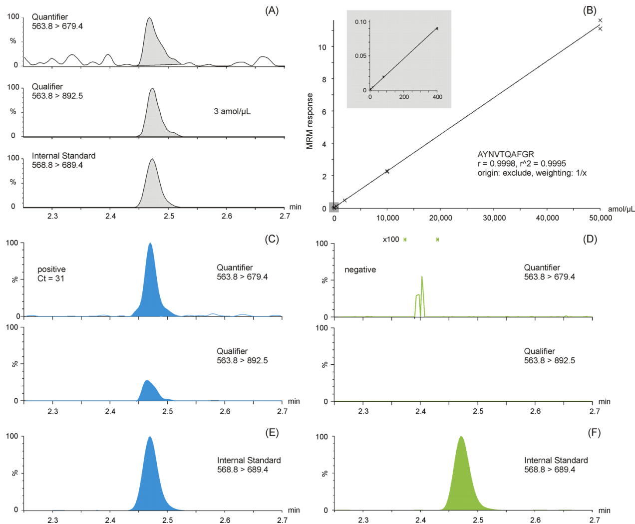
Figure 2. MRM chromatograms of antibody enriched NCAP AYNVTQAFGR peptide. Quantifier, Qualifier, and SIL Internal Standard peptide chromatograms spiked at the lower limit of quantification (3 amol/μl) (A) . Calibration curve of the AYNVTQAFGR peptide based on enriched recombinant NCAP protein digest, spiked with a constant amount of SIL peptide (B) . Two representative intensity-scaled MRM chromatograms of positive (mean Ct 31) (C) and negative (blank) (D) SARS-CoV-2 swab samples, respectively, normalized to the most abundant shared MRM transition. Intensity-scaled SIL Internal Standard peptide MRM chromatograms of positive (E) and negative (F) SARS-CoV-2 swab samples.
