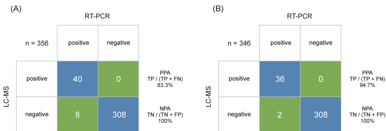
Figure 4. Output class (LC-MS) vs. target class (RT-PCR) contingency matrix, used to calculate the PPA and NPA of the SARS-CoV-2 immuno-affinity peptide enrichment LC-MS method (A) The LC-MRM/MS performance is based on RT-PCR results obtained from 48 positive and 308 negative samples. (B) The LC-MRM/MS performance based on all positive samples with a RT-PCR results below Ct 30 (LOD for the LC-MRM/MS) and 308 negative samples.
