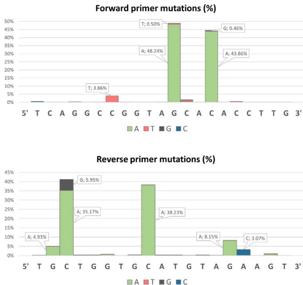
Fig. 1. Frequencies of single nucleotide mutations of SARS-CoV-2 homologous S gene sequences spanning a period from 21/1/2021 up to 19/4/2021 compared to primers SARSpUp2 and SARSpDo5.
