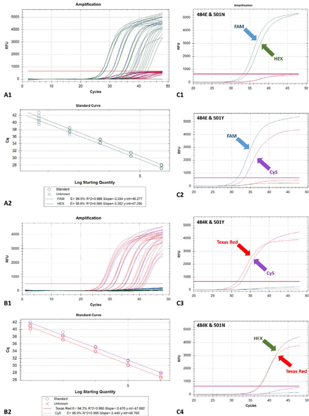
Fig. 2. (A1, B1) Amplification plots (fluorescence signals) generated by 2 dilution series of a WT strain (A; FAM/HEX fluorescence channels) and a South African variant strain (B; Texas Red/Cy5 fluorescence channels). Curves represent 10-fold serial dilutions, i.e. from left to right: 5 \times 10^5 down to 5 \times 10 copies/assay (WT, A1), and from 10^6 down to 10^2 copies/assay (South African variant, B1), each tested in 3 replicates. RFU: relative fluorescence units. (A2, B2) The corresponding standard curves. (C1-C4) Interpretation guide from testing representative SARS-CoV-2-positive samples, indicating all possible amino-acid substitution combinations (phenotypes) in the S protein 484 and 501 positions.
