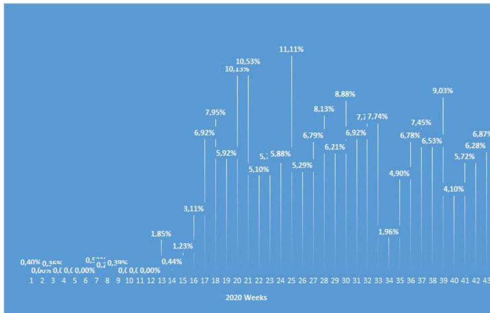
175 Fig 1. COVID-19 seropositive donation rate. 2020 evolution by weeks.
