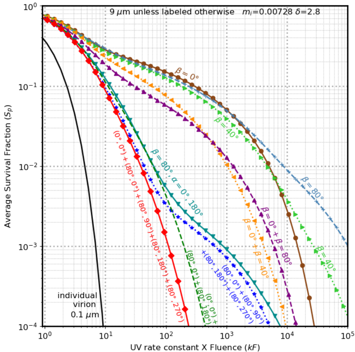
Figure 3. S_p vs kF , for 9- \mu\text{m} particles as in Fig. 1 (case with 260 nm illumination and \delta = 2.8 \mu\text{m} ), but with various combination of illumination beams. The three curves on the far right are each for a single illumination angle \beta : 0^\circ (solid, brown circles); 40^\circ (light green, dots and triangles); and 80^\circ (steel blue, dashed). The next two lines have an illumination wave normal to the surface ( \beta=0^\circ ) and a second wave at \beta=40^\circ (purple), or 80^\circ (dark yellow, dots, triangles). In each case, the total intensity illuminating the particle is the same.
