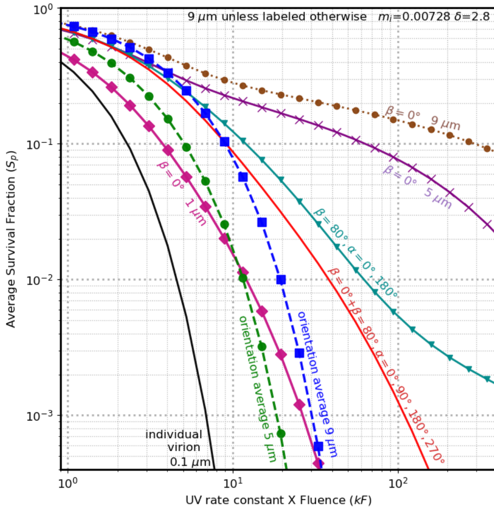
Figure 4. S_p vs kF for virions in particles as in Fig. 3 with 260-nm light, but the dashed lines are for particles illuminated with equal intensity from all directions (i.e., averaged over all orientations) with diameters ( d ) = 5 \mu\text{m} (green) and 9 \mu\text{m} (blue). Other cases are shown for particles illuminated with a wave propagating normal to the surface ( \beta=0^\circ ): individual virions (black); d = 1\text{-}\mu\text{m} (magenta diamonds), d = 5\text{-}\mu\text{m} (purple \times ), and d = 9\text{-}\mu\text{m} (brown circles with dotted line). Also shown from Fig. 3: five-beam case (solid red) and two beams with \beta = 80^\circ (cyan with triangles).
