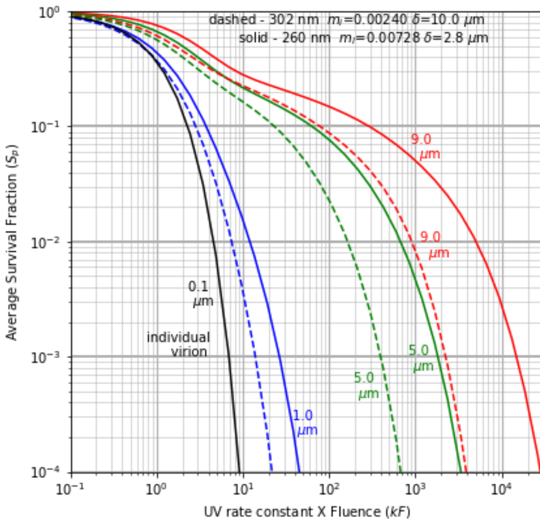
Figure 1. Average survival fractions ( S_p ) vs kF , the product of the UV rate constant ( k ) and the fluence ( F ) for 100 nm virions within spherical particles of dried respiratory fluids with the diameters indicated (9 \mu\text{m} , red; 5 \mu\text{m} , green; 1 \mu\text{m} , blue; 0.1 \mu\text{m} , black). The S_p at 260 nm are solid lines, and at 302 nm are dashed lines. Typically the k at 302 nm is less than the k at 260 nm. The particles are resting on a surface with real refractive index 1.4. The illuminating UV light propagates toward the surface in a direction perpendicular to the surface.
