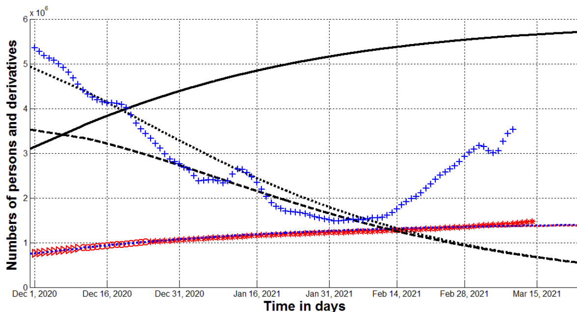
Figure. Visible (red) and real (black) COVID-19 epidemic dynamics in Ukraine.
