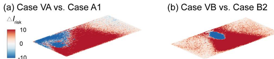
FIG. 13. Comparison of the I_{\text{risk}} map ( \Delta I_{\text{risk}} ) at the breathing level between the enhanced ventilation and optimal placement cases for the infector (a) in the front and (b) in the middle of the classroom with the air cleaner located near the HUV. The \Delta I_{\text{risk}} is defined as the I_{\text{risk}} of Case VA subtracted by that of Case A1 for (a) and the I_{\text{risk}} of Case VB subtracted by that of Case B2 for (b).
