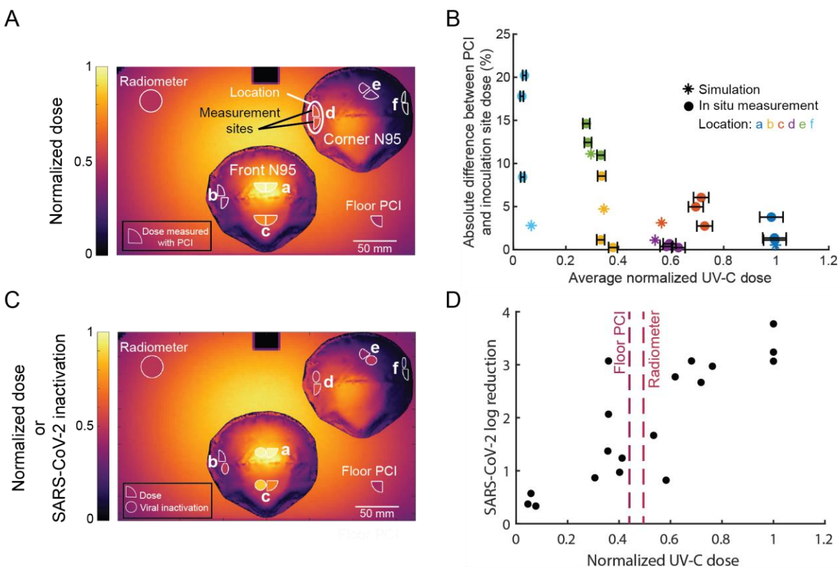
Figure 3: Paired on-N95 measurements of UV-C dose and SARS-CoV-2 inactivation show correlated, several-fold variation in dose and inactivation across one decontamination chamber. (A) Optical simulation of UV-C dose distribution over two 3M 1860 N95 facepieces in the UV-C chamber, overlaid with PCIs at paired measurement sites for viral inactivation and dose measurement. Heatmap shows simulated UV-C dose (normalized to the maximum dose in the chamber). PCI fill color represents the mean dose measured with PCIs in situ across triplicate measurements. (B) Comparison of dose differences within paired measurement sites. Data are colored by on-N95 location. Horizontal error bars on measured values represent the error in estimated dose. (C) Average normalized UV-C dose (quarter-circles) and SARS-CoV-2 inactivation (circles) at measured locations on front and corner N95, colored by the normalized value. Values are normalized to measurements at the apex of the front N95. Surrounding heatmap shows simulated UV-C dose. (D) SARS-CoV-2 inactivation on N95 facepieces is proportional to UV-C dose received. Selected locations on two N95 facepieces in the Spectronics XL-1000 UV-C chamber receive a 17.4 \pm 5.0 -fold difference in UV-C dose, which yields an 8.2 \pm 1.4 -fold difference in SARS-CoV-2 log reduction.
