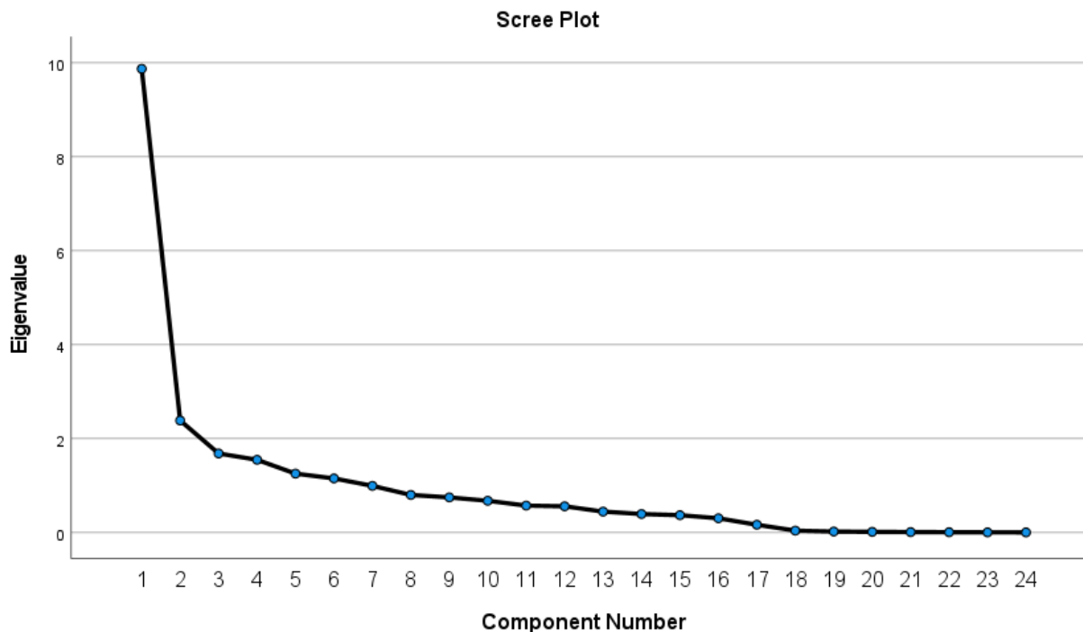
Figure 1: Scree plot
