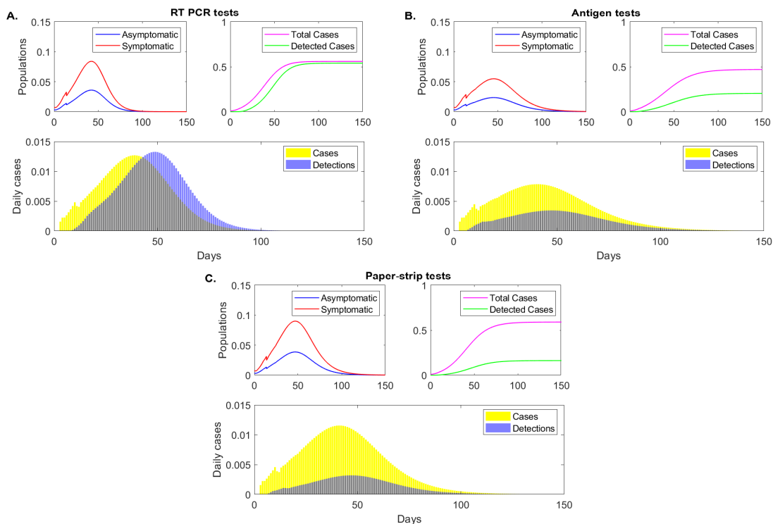
Figure 2: Epidemic dynamics over time. Sample epidemic dynamics results from varying testing regimes, as given by model eq. (5) for fixed testing capacity. Panel A: RT-PCR, detection threshold \log_{10}(V) = 2 , test return delay 5 days; Panel B: antigen test, detection threshold \log_{10}(V) = 5 , test return delay 0.5 days; Panel C: paper-strip test, detection threshold \log_{10}(V) = 6 , test return delay 0.1 days. Upper left figures: asymptomatic (blue), symptomatic (red) populations over time. Upper right figures: cumulative positive cases (magenta) and cumulative detected cases (green) over time. Lower figures: daily new cases (yellow bars) and daily new case detections (blue bars).
