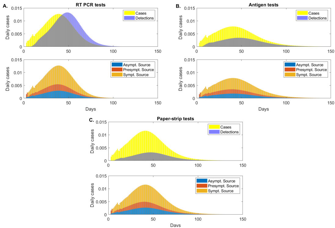
Figure 4: Asymptomatic, presymptomatic and symptomatic transmissions. (Upper figures): daily cases (yellow bars) and daily detections (blue bars); (Lower figures): daily cases due to asymptomatic transmission (blue bars), presymptomatic transmission (red bars) and symptomatic transmission (orange bars), as given by model eq. (5) for fixed testing capacity. Panel A: RT-PCR, detection threshold \log_{10}(V) = 2 , test return delay 5 days; Panel B: antigen test, detection threshold \log_{10}(V) = 5 , test return delay 0.5 days; Panel C: paper-strip test, detection threshold \log_{10}(V) = 6 , test return delay 0.1 days.
