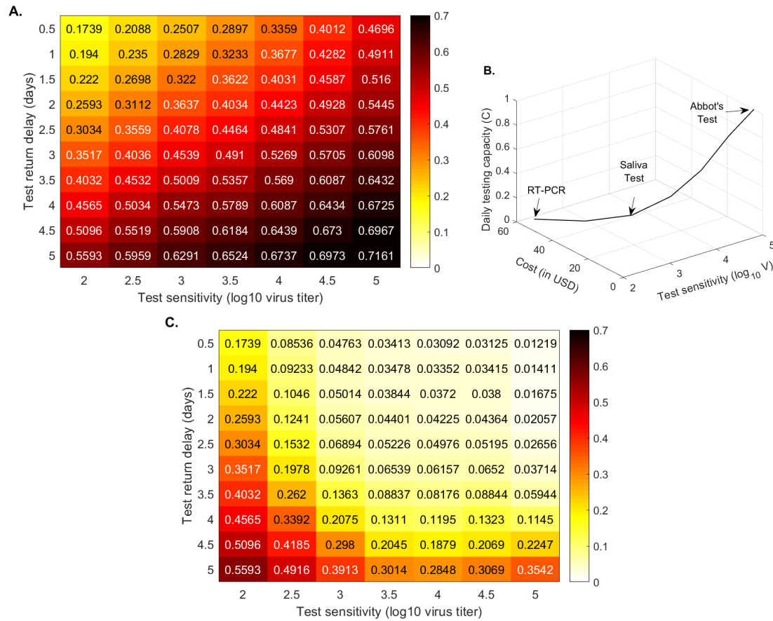
Figure 3: Cumulative cases at half a year. Heatmaps for the cumulative cases at half a year after the outbreak (% of the total population) as given by model eq. (5) versus test sensitivity and test return delay. Panel A: fixed testing capacity per day, C = 0.1 . Panel B: relationship between capacity and cost. Panel C: fixed testing budget per day. Parameters and initial conditions are given in Tables 1 and 2.
