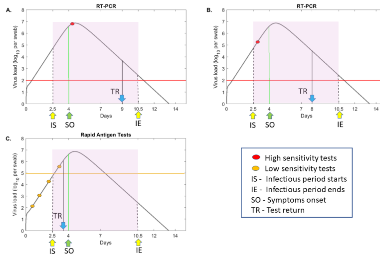
Figure 1: RT-PCR versus rapid testing practices. \log_{10} virus load per swab over time as given by model (1) (grey curves) for values in [20]. Patients are assumed to be infectious from t = 2.5 days (IS) till t = 10.5 days (IE) (shaded region) and symptomatic beginning on day t = 4 (SO). Panels A and B depict testing with a high-sensitivity RT-PCR test with detection threshold \log_{10}(V) = 2 per swab (red line) and test return delay of five days. In panel A, the test occurs immediately following symptoms onset, and in panel B, the test occurs before symptoms onset (red circles). Panel C depicts frequent testing (yellow circles) with a low-sensitivity test with detection threshold \log_{10}(V) = 5 per swab (yellow line) and test return delay of one half day. TR shows the time of positive test result.
