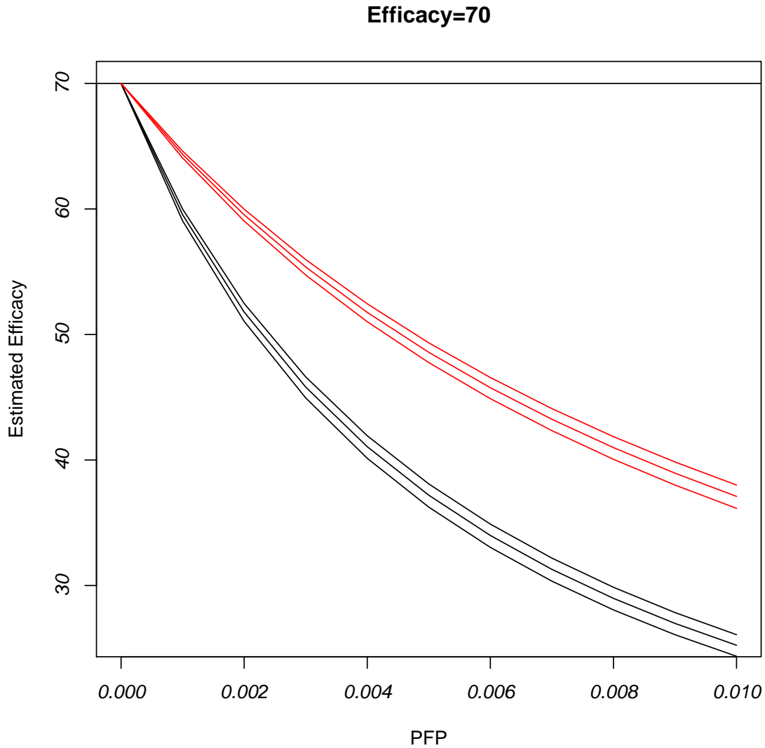
Figure 2: Illustration of bias due to misclassification at efficacy = 70% (solid horizontal line). Plot of what is estimated (on average) using the observed rates as a function of PFP. Black lines are for different PFN (.025, .05 and .10) based on \pi_p = .006 with \pi_v = .0018 . Red lines are based on \pi_p = .012 with \pi_v = .0036 .
