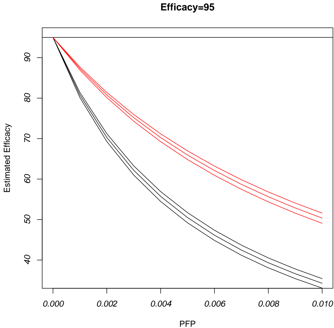
Figure 1: Illustration of bias due to misclassification at efficacy = 95% (solid horizontal line). Plot of what is estimated (on average) using the observed rates as a function of PFP. Black lines are for different PFN (.025, .05 and .10) based on \pi_p = .006 with \pi_v = .0003 . Red lines are based on \pi_p = .012 with \pi_v = .0006 .
