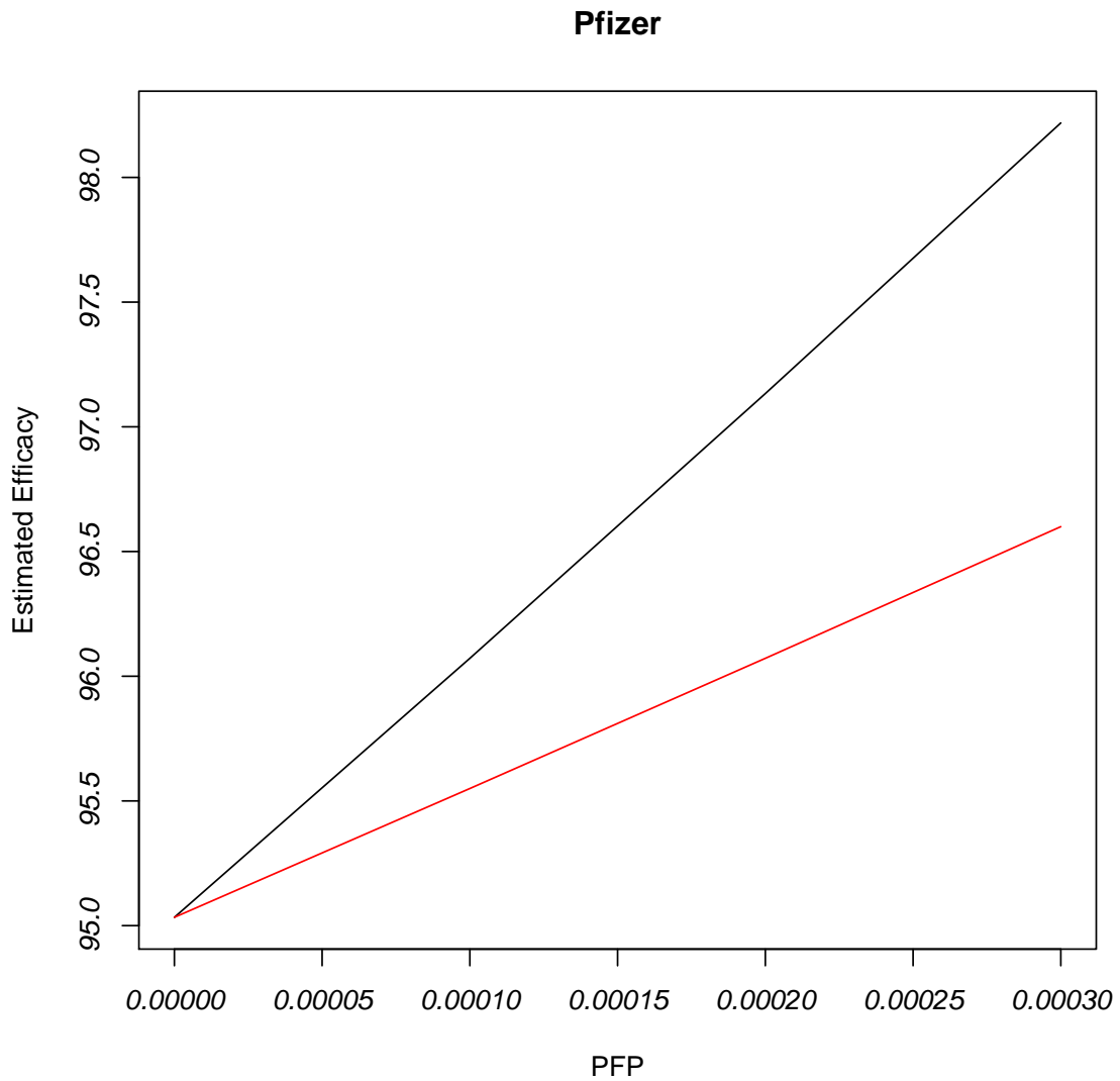
Figure 5: Illustration of correction of estimated efficacy with the Pfizer data as a function of possible values of PFP. Black line uses the original data while red line is with doubled positive rates. Original estimated efficacy equals 95.04% in each case
