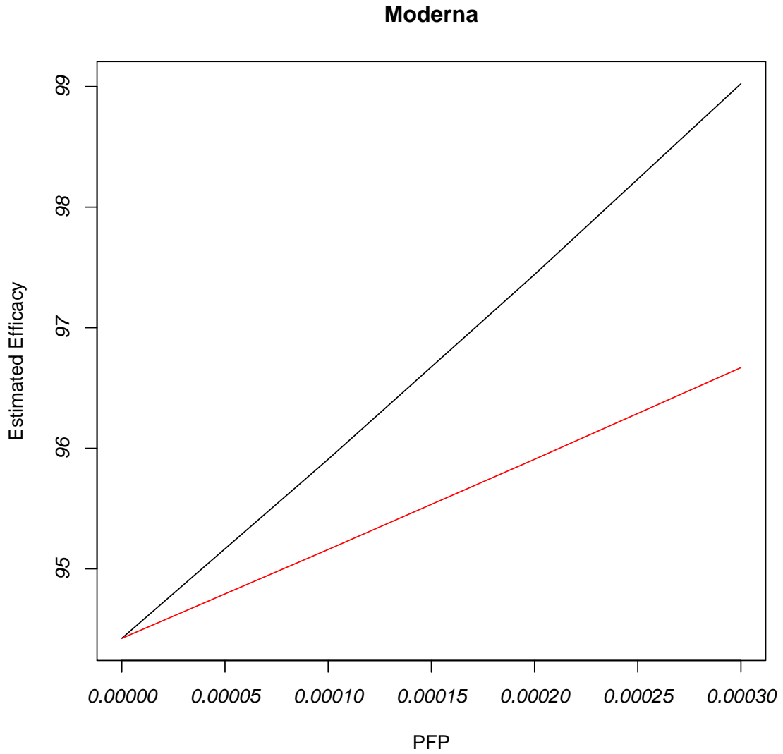
Figure 4: Illustration of correction of estimated efficacy with the Moderna data as a function of possible values of PFP. Black line uses the original data while red line is with doubled positive rates. Original estimated efficacy equals 94.4% in each case
