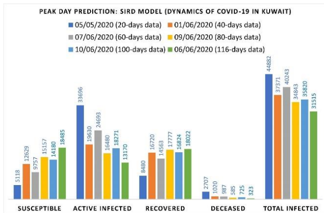
(a) SIRD model - peak day
