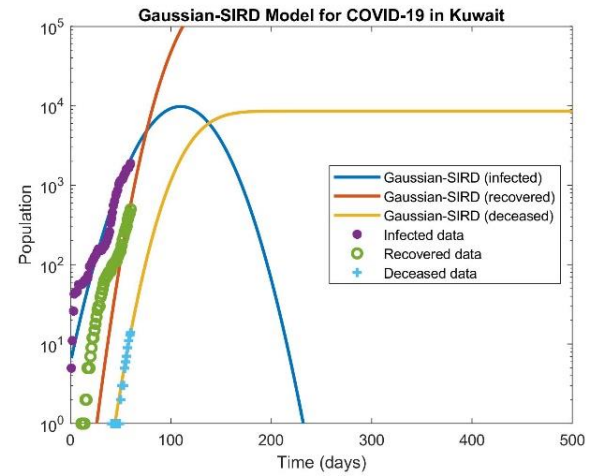
(f) 60-days Gaussian-SIRD Model
