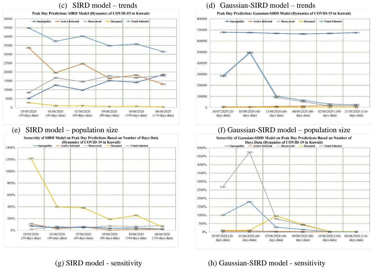
Figure 2. Comparison of SIRD and Gaussian-SIRD models on precision and sensitivity for predicting peak day of infection using 20, 40, 60, 80, 100, and 116 subsequent days of COVID-19 data in Kuwait (18 June 2020).
