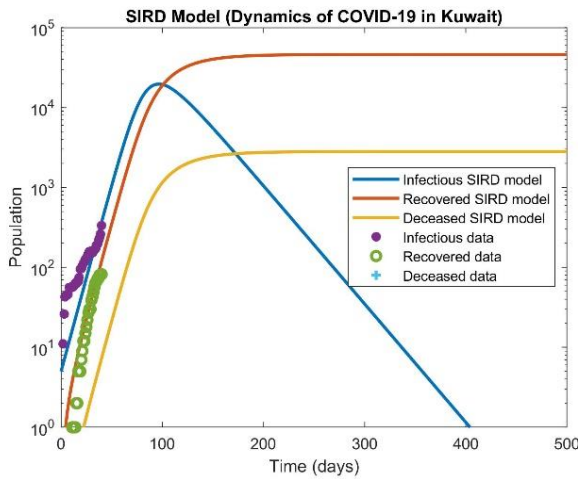
(c) 40-days SIRD Model
