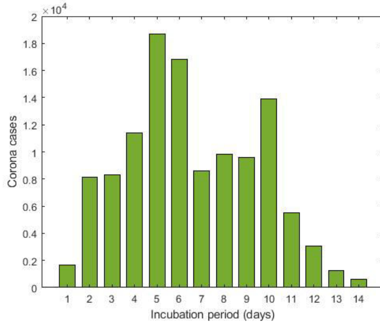
Figure 3: The cumulative data of confirmed corona cases for first 200 days is splitted into several incubation periods.
