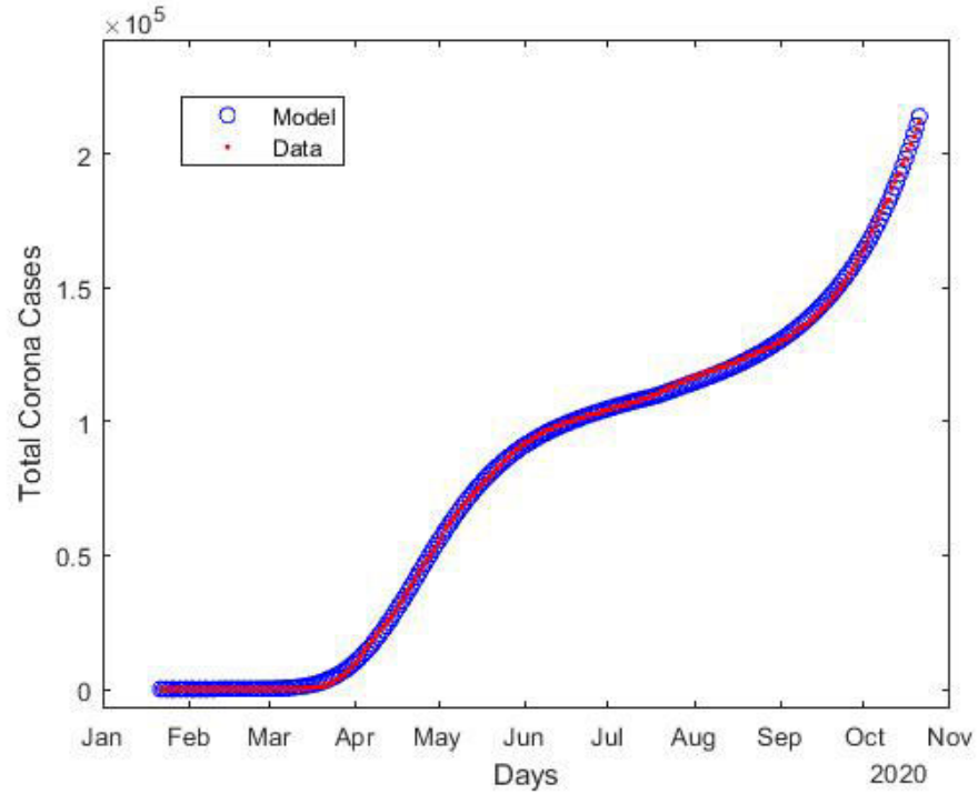
Figure 1: Estimation of the total number of confirmed coronavirus cases ( T ) compared to the available data ( I ). Here blue circles indicates the results obtained from model, and red line is the publicly available data ( I ).
