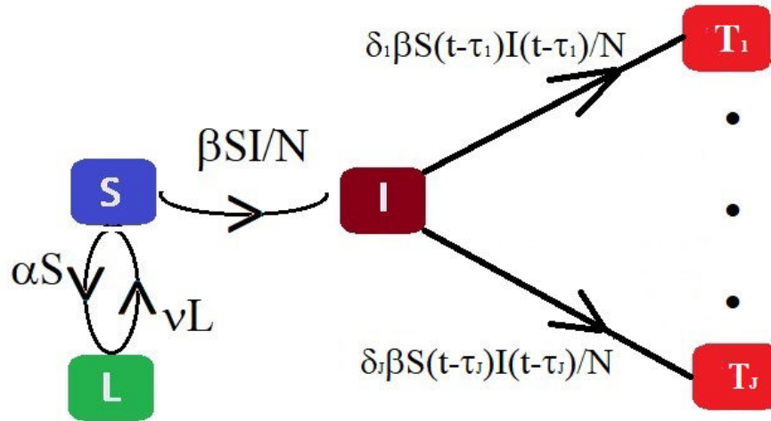
Figure 1: Schematic diagram of the compartmental based epidemic model, presented in Equation 2.
