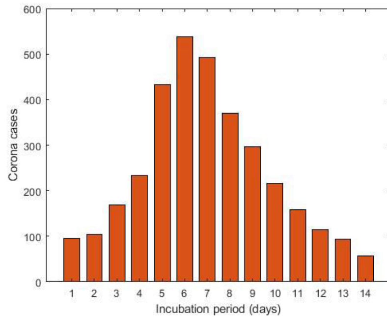
Figure 4: The confirmed corona cases as of October 23, 2020 is splitted into several incubation periods.
