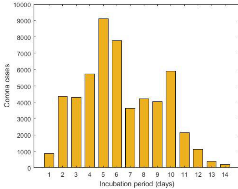
Figure 2: The cumulative data of confirmed corona cases for first 100 days is splitted into several incubation periods.
