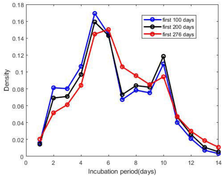
Figure 3: Probability densities of incubation period, presented in Eqn. 8 . The 'first 100 days' indicates that the density of incubation period based on the cumulative data of the first 100 days during the epidemic starting from January 22, 2020 and similar for other two.
