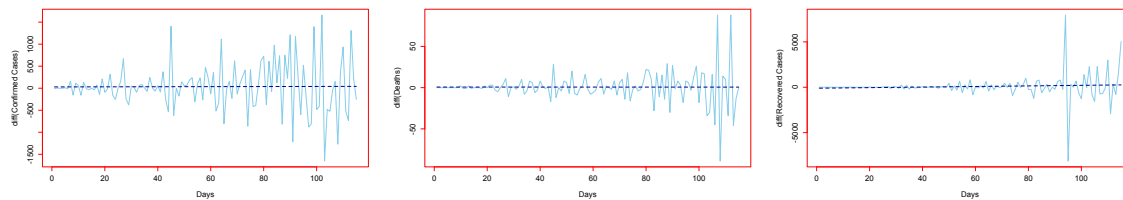
Figure 2: Differenced series: 1st order difference for Confirmed ( left ), Deaths ( middle ) and Recovered cases ( right ).
