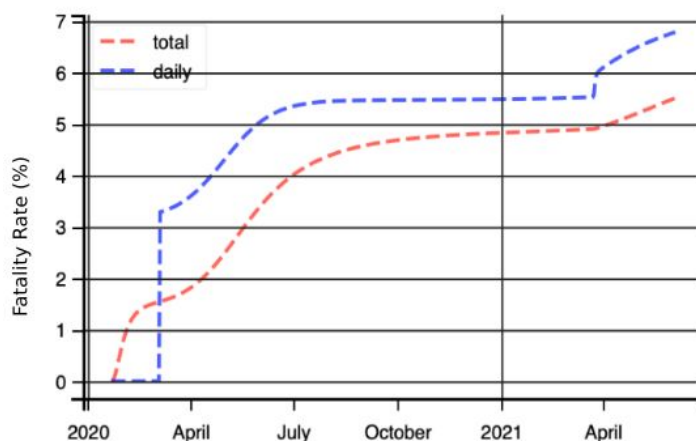
Figure 1: Fatality Rate Projection with time for India
