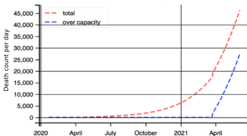
Figure 3: Death per day projection with time for India
