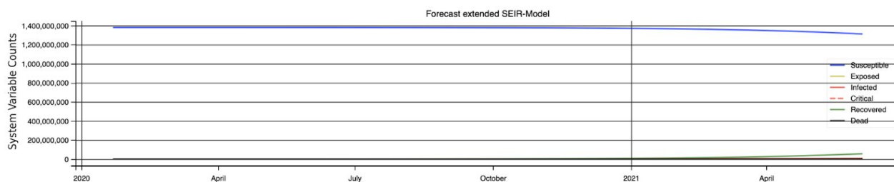
Figure: Extended SEIR Compartment Count Projection till May 2021
