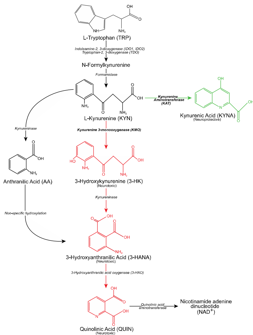
Figure 1 Overview of the kynurenine pathway. Adapted with authors and editors' permission (1). The designations 'neurotoxic' and 'neuroprotective' are assigned on the basis of the balance of evidence and are acknowledged to be simplifications of complex properties.
