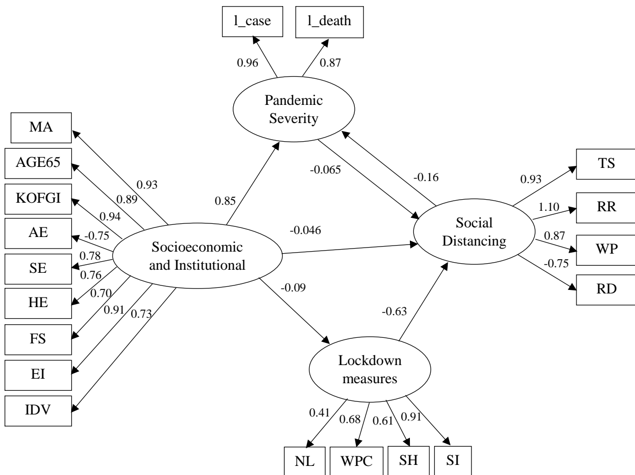
Figure 3: The calibrated model with direct standardized effects
