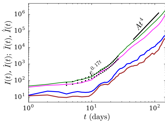
Fig. 4 (color online) The log-log plot of total infected individual vs. time for India (both cases, see Table 3). Both I(t) (green curve) and \bar{I}(t) (magenta curve) curves follow a power-law, i.e., I(t) = At^4 , where A = 0.007 . The thick blue and brown curves in the plot depict the derivatives of I(t) and \bar{I}(t) respectively.
