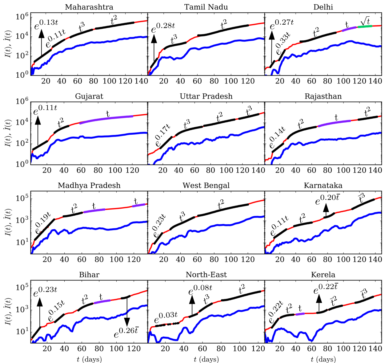
Fig. 1 (color online) The semi-log plots of total infection count ( I(t) ) vs. time ( t ) (red thin curves) and \dot{I}(t) vs. t (blue thick curves) for the eleven states individually and consolidated for north-eastern Indian states. The dotted curves represent the best-fit curves. Refer Table 1 for the best-fit functions.
