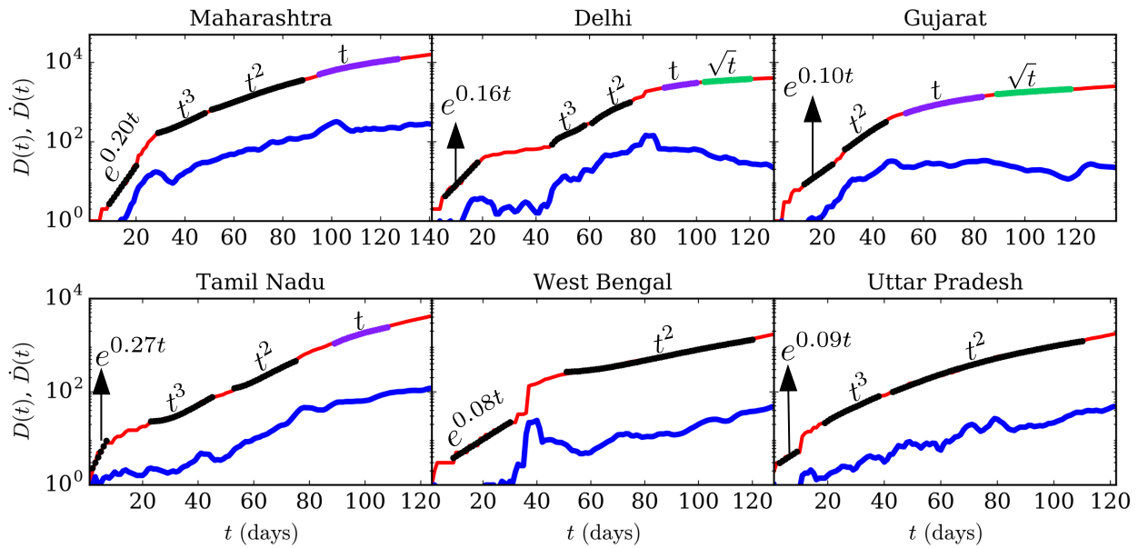
Fig. 2 (color online) The semi-log plots of total death cases ( D(t) ) vs. time ( t ) (red thin curves) and \dot{D}(t) vs. t (blue thick curves) for six states of India. The dotted curves represent the best-fit curves (see Table 2).
