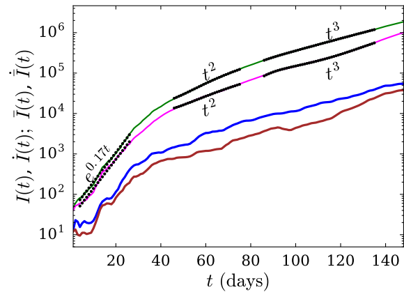
Fig. 3 (color online) The semi-log plot of total Infection count ( I(t) ) vs. time ( t ) curves for India (green curve) and India other than Maharashtra, Tamil Nadu and Delhi (magenta curve) where, \bar{I}(t) = I(t)_{IND} - \{I(t)_{MH} + I(t)_{TN} + I(t)_{DL}\} . The thick blue and brown curves in the plot depict the derivatives of I(t) and \bar{I}(t) respectively. The dotted curves represent the best-fit curves.
