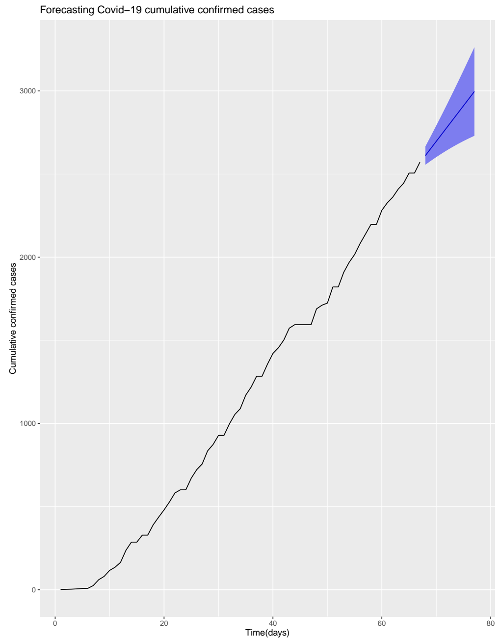
Fig 2. Forecasts with 95% prediction interval.
