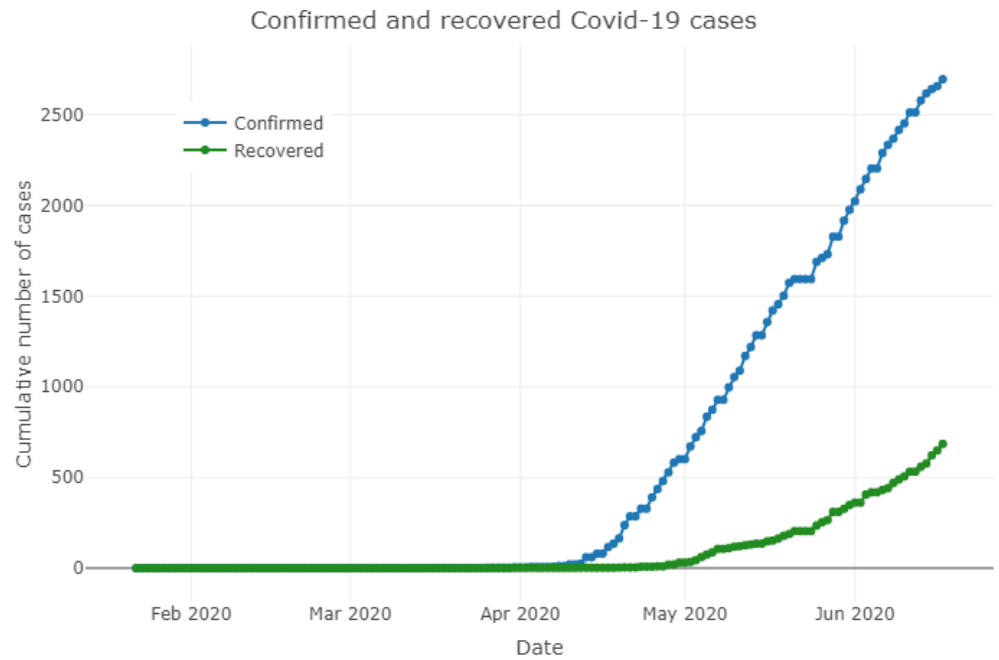
Fig 1. Cumulative confirmed and recovered Covid-19 cases in Somalia.
