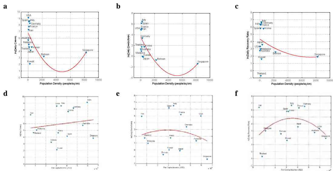
Fig.1. Effect of Socio-economic factors on the COVID-19 parameters , i.e. relationship between (a, b, c) population density, (d, e, f) per capita income vs. daily cases, death rate and recovery rate, respectively. Correlation accuracy evaluation is listed in Table S5 .
