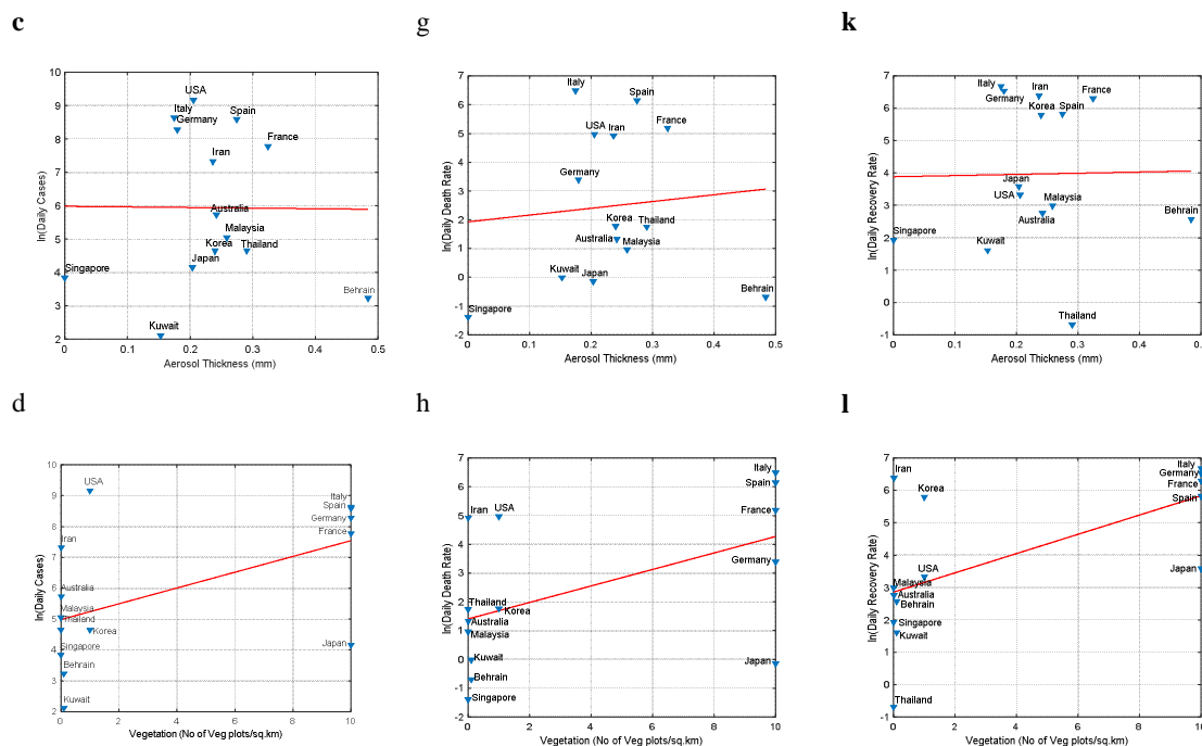
Fig.3. Effect of Natural factors on the selected COVID-19 parameters , i.e. relationship between (a, e, i) temperature, (b, f, j) relative humidity, (c, g, k) aerosol, (d, h, l) vegetation vs. daily cases, death rate and recovery rate, respectively. Correlation accuracy evaluation is listed in Table S5 .
