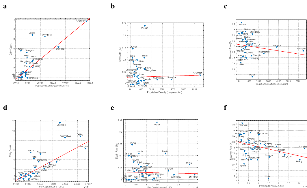
Fig.4. Effect of Socio-economic factors on the COVID-19 parameters, i.e. relationship between (a, b, c) population density, (d, e, f) per capita income vs. daily cases, death rate and recovery rate, respectively.
