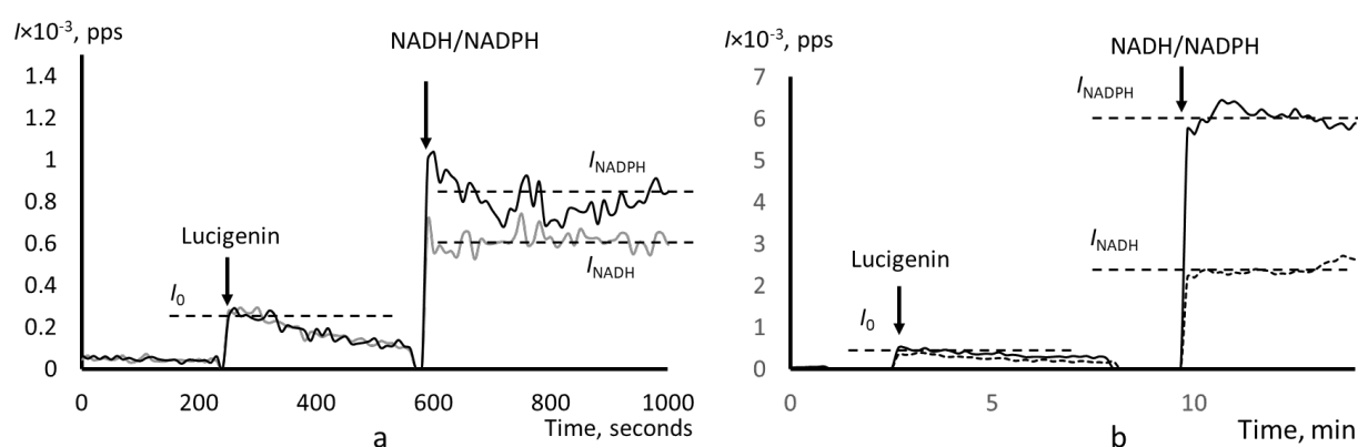
Figure 1. Chemiluminograms of thyroid tissue samples: (a) euthyroid goiter; (b) PTC, a patient with high activity of microsomal reductases; the analytical parameters and time of addition of lucigenin and NADH/NADPH are shown in the figure.
