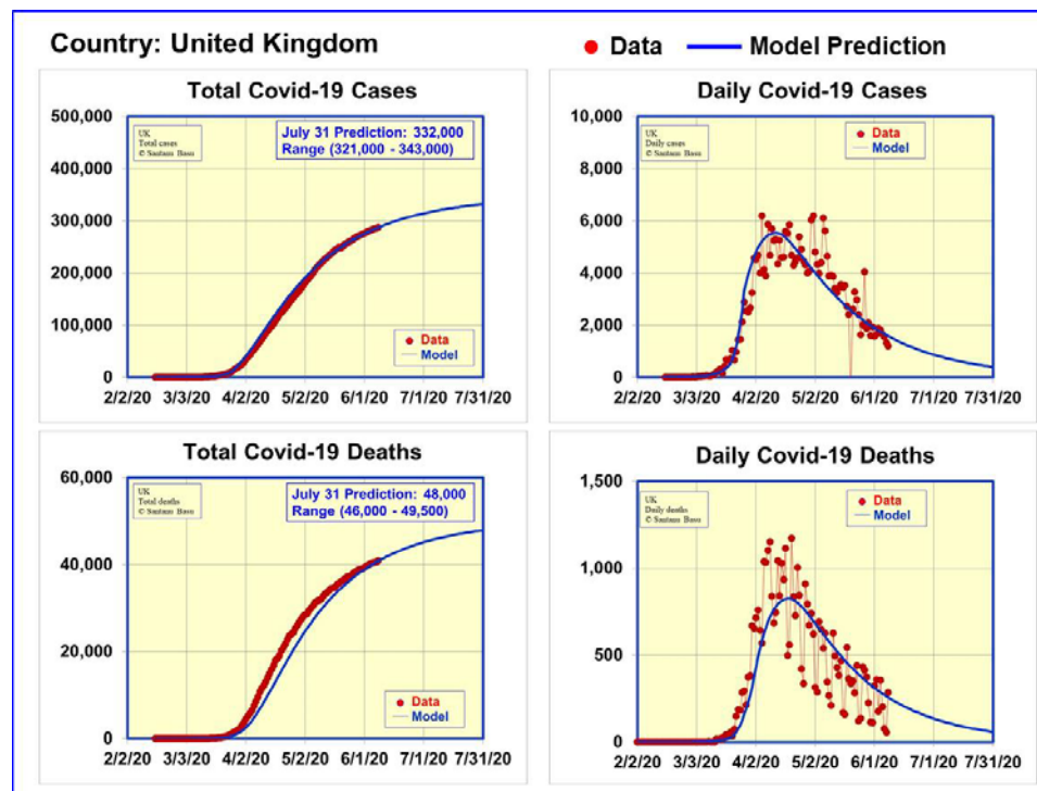
Figure 1. Data and model predictions for Covid-19 cases and deaths in the UK
