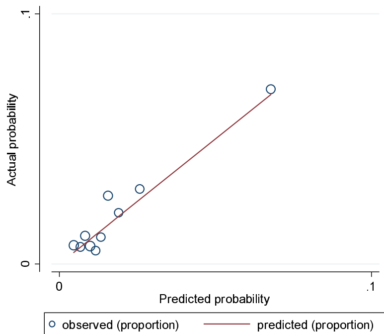
Figure 5. A calibration plot with distribution of the predicted probabilities for individuals with and without in-hospital bleeding in the validation data sets.
