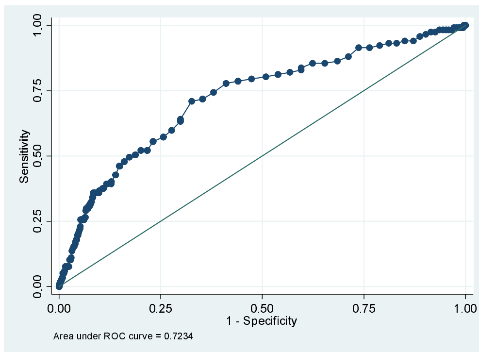
Figure 4. Receiver-operating characteristics curve in identifying patients with in-hospital bleeding in the validation data sets
