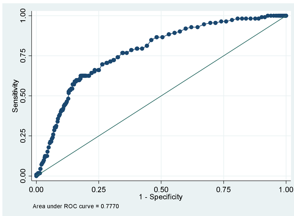
Figure 2. Receiver-operating characteristics curve in identifying patients with in-hospital bleeding in the development dataset.
