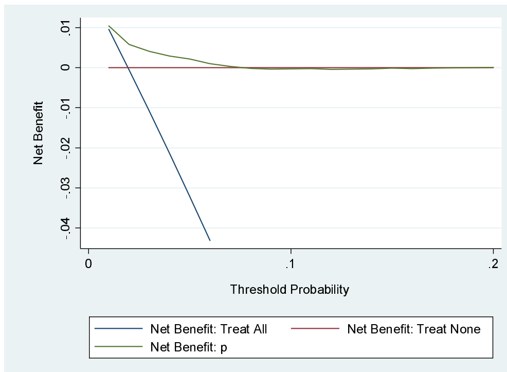
Figure 6. DCA in the validation data sets.
