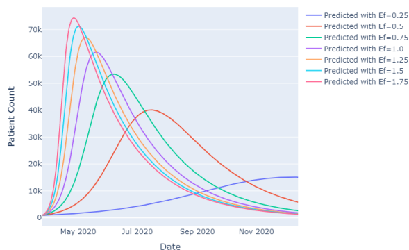
Figure 7. SIR modelling infected patients prediction
