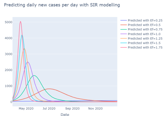
Figure 11. Daily new cases/day predicted by SIR model
