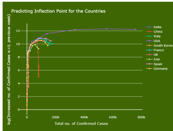
Figure 10. Country-wise inflection point analysis on COVID-19 data
