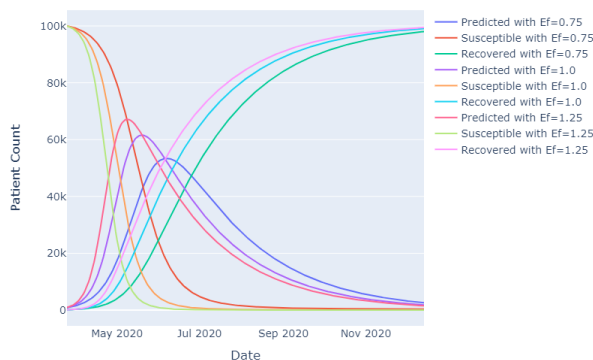
Figure 9. SIR modelling with restriction impact factor E_f
