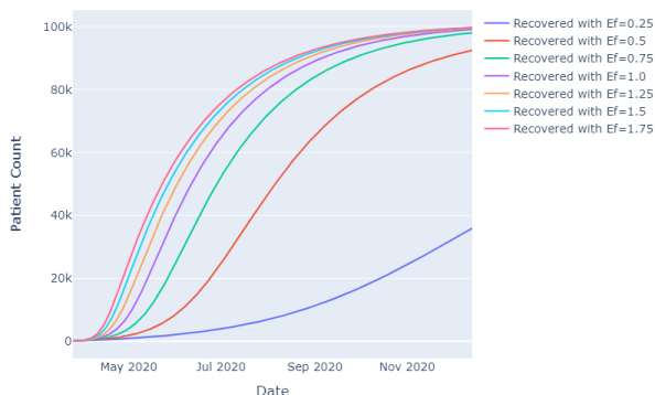
Figure 8. SIR modelling recovered patients prediction
