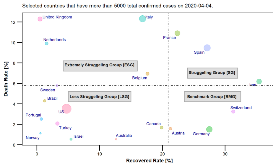
Figure 11: The Death Rate - Recovered Rate Matrix.
