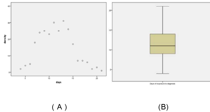
Figure 2 Time distribution of nucleic acid positive from exposure to first swab of pharynx(A is a scatterplot , B is a boxplot)
