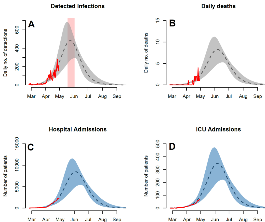
Figure 3. Observed and forecasted trajectories assuming 500,000 susceptibles. Observed and projected daily numbers of A) incident infections, B) death cases, C) general hospital admissions and D) ICU admissions. Red rectangular ribbon highlights the projected time-window of the epidemic peak. Red lines represent the reported data. Black dashed lines represent model projections based on MLE of unknown parameters with shaded ribbons representing 95% credible interval on new observations. We note here that the observed cases and their projections only represent a fraction of the actual and model prevalence. This is based on our assumption of under-reporting and the presence of asymptomatic individuals in the population.
