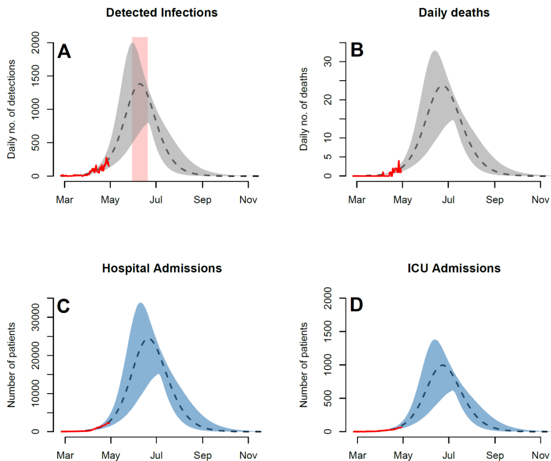
Figure 4. Tripling the size of the susceptible population. Peaks of forecasted trajectories are approximately tripled in size. The projected time-window of the peak is delayed by 2-weeks and widened (3-week period). Observed and projected daily numbers of A) incident infections, B) death cases, C) general hospital admissions and D) ICU admissions. Red rectangular ribbon highlights the projected time-window of the epidemic peak. Red lines represent the reported data. Black dashed lines represent model projections based on MLE of unknown parameters with shaded ribbons representing 95% credible interval on new observations. We note here that the observed cases and their projections only represent a fraction of the actual and model prevalence. This is based on our assumption of under-reporting and the presence of asymptomatic individuals in the population.
