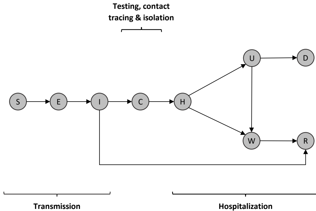
Figure 2. Schematic diagram of the CoVID-19 transmission model. Individuals (S) susceptible to the virus become infected by infectious individuals (I) at rate. They then move through a latent period (E) at rate before becoming infectious (I). Infectious individuals can either move through a detection period (C) at a rate or eventually recover without symptoms at a rate. Confirmed infectious individuals move through an initial hospitalization period (H) at a rate after which they are admitted to either an isolation ward (W) at a rate or an intensive care unit (U) at a rate. Intensive care patients may recover and be sent to an isolation ward W at a rate or ultimately die (D) at a rate. Isolated patients move through a recovery period (R) at a rate, where they are assumed to be immune to the disease, at least in the medium term.
