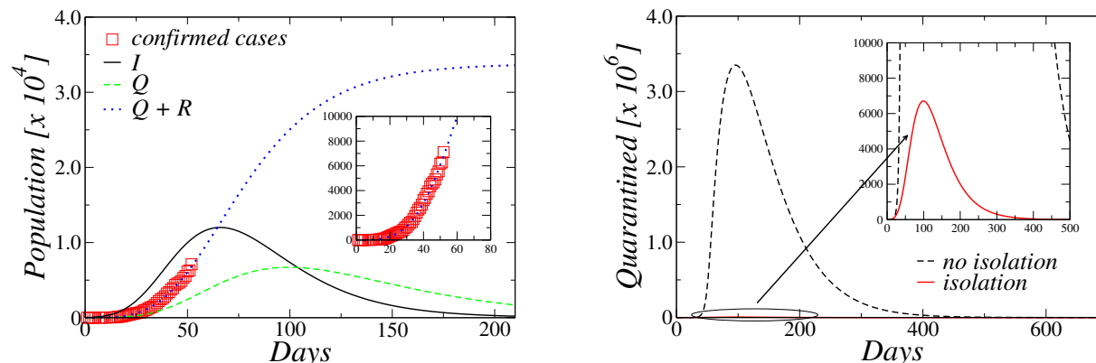
FIG. 4. (Color online) Left panel : Time evolution of the number of Infected (I), Quarantined (Q) and total confirmed cases (Q+R) considering all the data and isolation policies, obtained by the numerical integration of Eqs. (8) to (11). Data of confirmed cases are exhibited as well (squares). In the inset we show a zoom in the region of the current data (from March 5, 2020 through April 26, 2020), to highlight the agreement of the model with the data. Right panel : Flattening the curve: comparison between the predicted number of Quarantined individuals for the model with (full line) and without (dashed line) the implementation of isolation policies. The peak of the curve is considerably reduced. In both figures the parameters are I_0 = 24 , \beta = 0.32 , \eta = \alpha = 0.018 , k_0 = 0.033 and \gamma = 0.02 .
