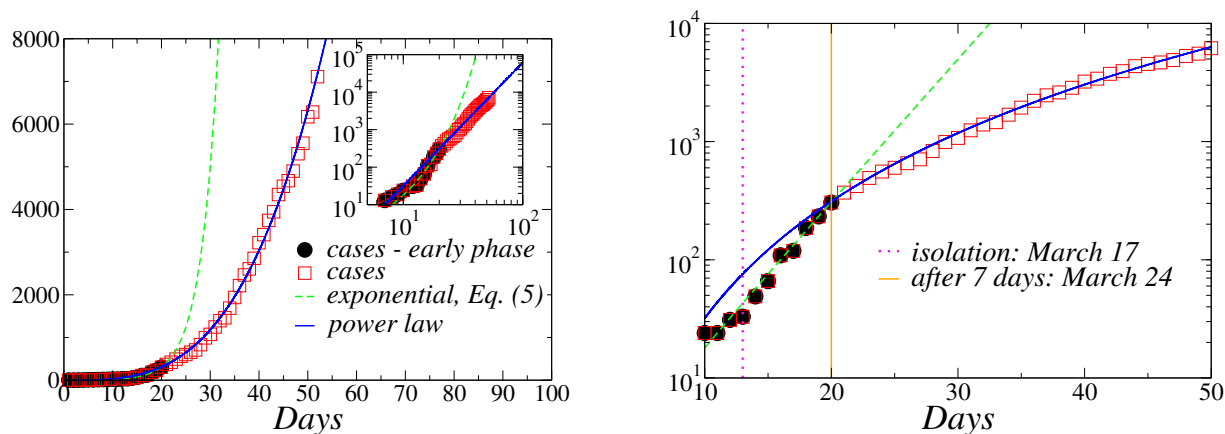
FIG. 3. (Color online) Left panel : Time evolution of the total number of confirmed cases from March 5, 2020 through April 26, 2020 (squares). The dashed line is given by Eq. (5). As a guide to the eyes, we also show a power law fit of the data (full line). In the inset we exhibit the same data in the log-log scale. Right panel : Log-linear plot of the same quantities. The vertical dotted line marks the beginning of the isolation policies in Rio de Janeiro (March 17, 2020). One can see that the social distancing policies changed the initial exponential growth after 7 days (March 24, 2020).
