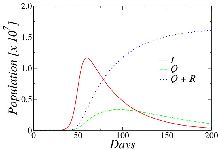
FIG. 2. (Color online) Time evolution of the number of Infected ( I ), Quarantined ( Q ) and total confirmed cases ( Q+R ) predicted by the SIQR model, for the initial epidemic phase, obtained by the numerical integration of Eqs. (1) to (4). The parameters are I_0 = 13 , \beta = 0.3036 , \eta = \alpha = 0.0127 and \gamma = 0.02 .
