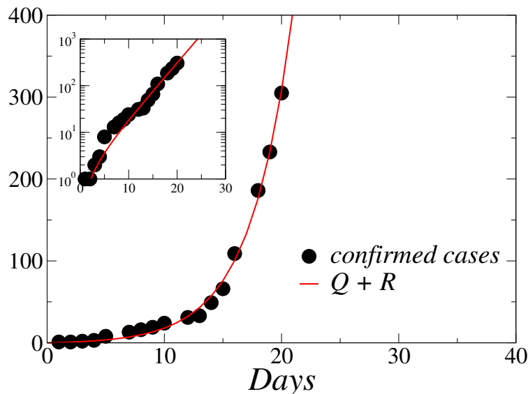
FIG. 1. (Color online) Comparison between the number of confirmed cases in Rio de Janeiro state (circles) and Eq. (5) (full line), for the initial epidemic phase. The parameters are I_0 = 13 , \beta = 0.3036 , \alpha + \eta = 0.0254 , as discussed in the text. In the inset we exhibit the graphic in the log-linear scale, showing the typical linear behavior of the exponential function.
