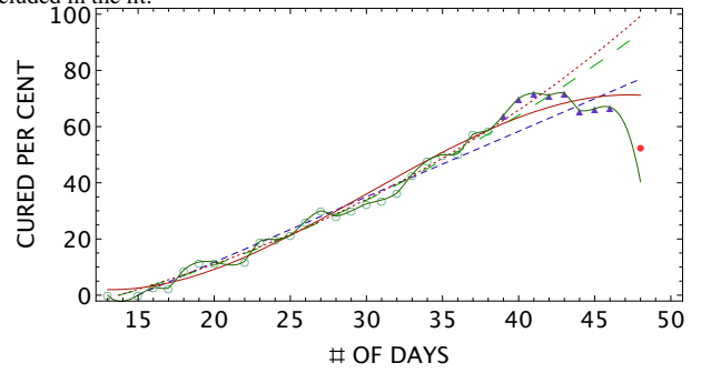
Figure 9: The same as in Fig. 8 but for the per cent number of cured persons. The data come from Table 3. Green circles are data until 38 days. Blue triangles are new data until 46 days. Red points are data from 48 days not included in the fit.
