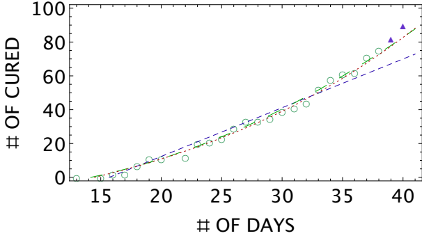
Figure 6: Comparison of different model predictions using the data in Table 3. The dashed blue line is a linear fit. The long dashed green curve is a quadratic fit. The dot red curve is the prediction of the modified SI-like model in [10, 11]. Green circles are data until 38 days. Blue triangles are new data for 39 and 40 days not included in the fitting procedure.
