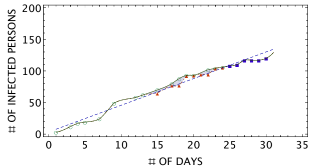
Figure 2: Number of infected persons versus the number of days : green circles are the input data from [2, 5]. The red triangles are data from [6] from the 17th day. Blue rectangles are new data [2, 5, 6] from 25th to 30th days. The continuous olive curve is the fit from 1 to 30th days of [2, 5] data while the red dot-dashed one is the fit of [6] data which follows the red triangles data points. The dashed blue line is the linear fit given in Eq. 2.
