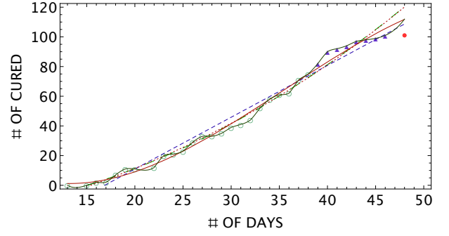
Figure 8: Comparison of different model predictions using the data in Table 3. The dashed blue line is a linear fit. The long dashed green curve is a quadratic fit in Eq. 4. The dot red curve is the prediction of the SI-like model in [10, 11]. The continuous red curve is the cubic polynomial fit. The continuous oliva curve is the result from a least \chi^2 -fit. Green circles are data until 38 days. Blue triangles are new data until 46 days. Red points are data from 48 days not included in the fit.
