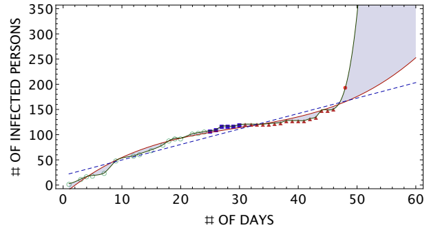
Figure 5: Data are the same as in Fig 4. New fit including the new data 193 (red point) on 7 may from [6]. The oliva curve is the \chi^2 -fit. The continuous red curve is the cubic polynomial. The dashed line is the linear fit.
