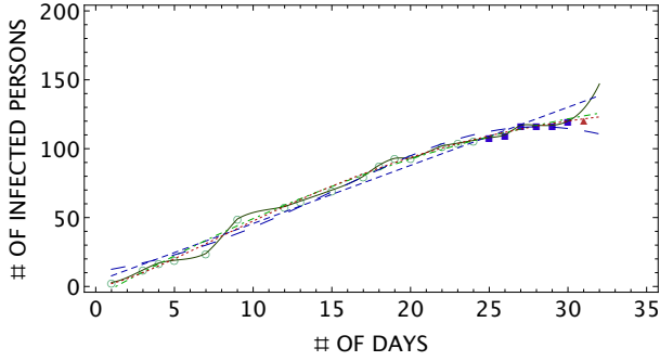
Figure 3: Data are the same as in Fig 2. New data (red triangle) is not included in the fit. The continuous oliva curve is the fit from 1 to 25th days of [2, 5] data and 25th to 30th days of data from [2, 5, 6]. The dashed blue line is the linear fit in Eq. 3 while the dot-dashed green curve is the quadratic fit given in Eq. 4. The dotdashed red curve is the fit from the SI-like model used in [10, 11] while the large dashed green curve is the one from a gaussian-like fit used in [22].
