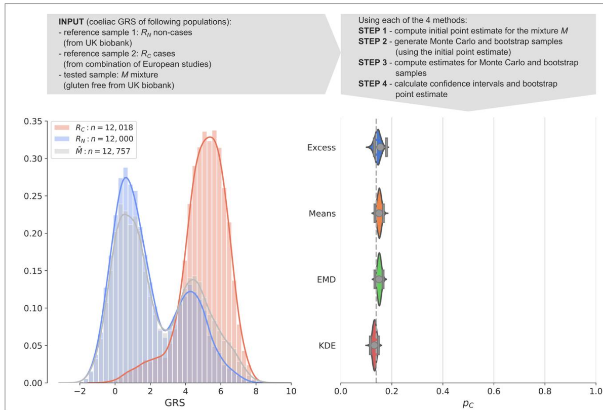
Figure 5: Coeliac disease dataset worked example. A comparison of the four methods applied to a gluten-free cohort from the UK biobank (mixture population \tilde{M} ). The reference and the mixture distributions are plotted on the left ( R_C , shaded red, R_N , shaded blue, \tilde{M} , shaded grey, respectively). Estimated values of prevalence p_C and 95% confidence intervals (grey dots and lines with bars at the ends) are plotted on the right showing estimates of Excess = 15.5%, Means = 15.0%, EMD = 15.0%, KDE = 13.2%. The violin plots show the distribution of the 100,000 estimates of prevalence ( p'_C ) in the bootstrap samples. The proportion of participants adhering to a gluten-free diet and reporting coeliac disease is shown as a dashed vertical line. Calculations were based on the following participants: non-cases UK Biobank, cases coeliac disease reference cohort, mixture self-reported gluten-free diet UK Biobank.
