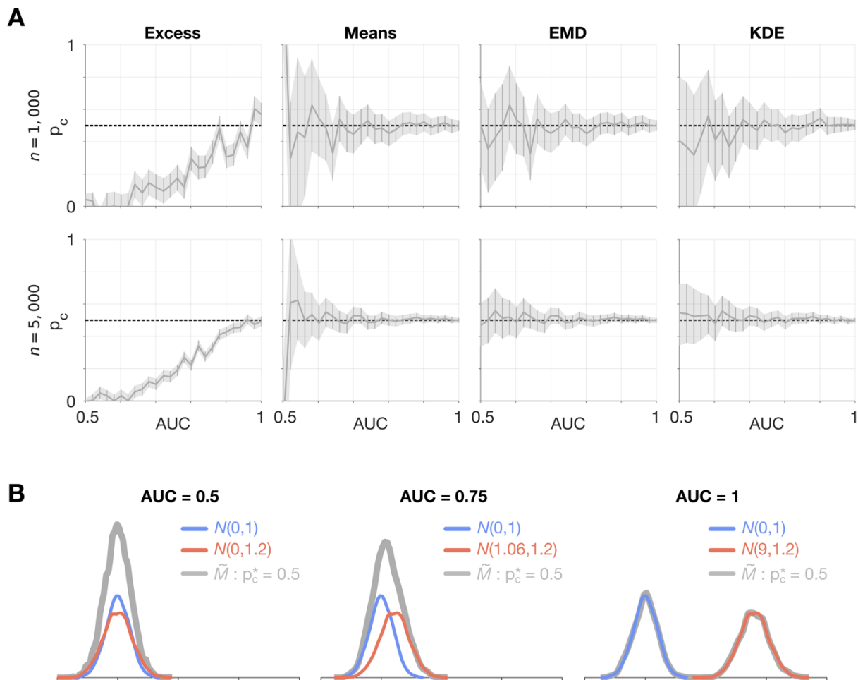
Figure 4: A comparison of the four methods using an artificial genetic risk score with increasing discriminative ability as measured by AUC, from AUC = 0.5 (no discriminative ability) through to AUC = 1, (complete differentiation). The estimated proportion with confidence intervals for each of the methods (Excess, Means, EMD, KDE) are shown using mixture populations with sample size, n = \{1000, 5000\} . This figure is generated using artificial data: N(\mu, \sigma) is a normal distribution with mean \mu and standard deviation \sigma and \tilde{M} is an equal mixture of the two normal distributions ( p_c^* = 0.5 ).
