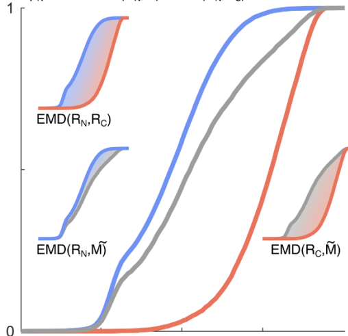
Figure 2: Illustration of the four proportion estimation methods. Each method uses different characteristics of the mixture and reference populations to estimate the proportion of constituents of the mixture population ( p_C and p_N ). The Excess method (A) considers the number of cases above the mixture median in excess of those expected in a pure disease reference population. The Means method (B) uses the normalised difference of the mixture population's mean and the two reference populations' means. The earth mover's distance method (C) uses the weighted costs of transforming the mixture distribution into the reference populations. The Kernel density estimation method (D) fits smoothed templates to each of the reference populations and then fits a weighted sum of these templates to the mixture population, adjusting the amplitudes of each with the Levenberg–Marquardt algorithm. Figure generated using artificial data.
