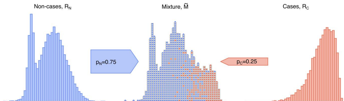
Figure 1: Illustration of a mixture population drawn from two reference populations. This emulates the real-world scenario of a population composed solely of individuals drawn from each subpopulation of non-cases ( R_N , blue) and cases ( R_C , red). Data are sampled with replacement from the two depicted reference populations to generate a mixture ( \tilde{M} ) population of a particular sample size and proportion, which possesses features of both reference populations. Figure generated using artificial data.
