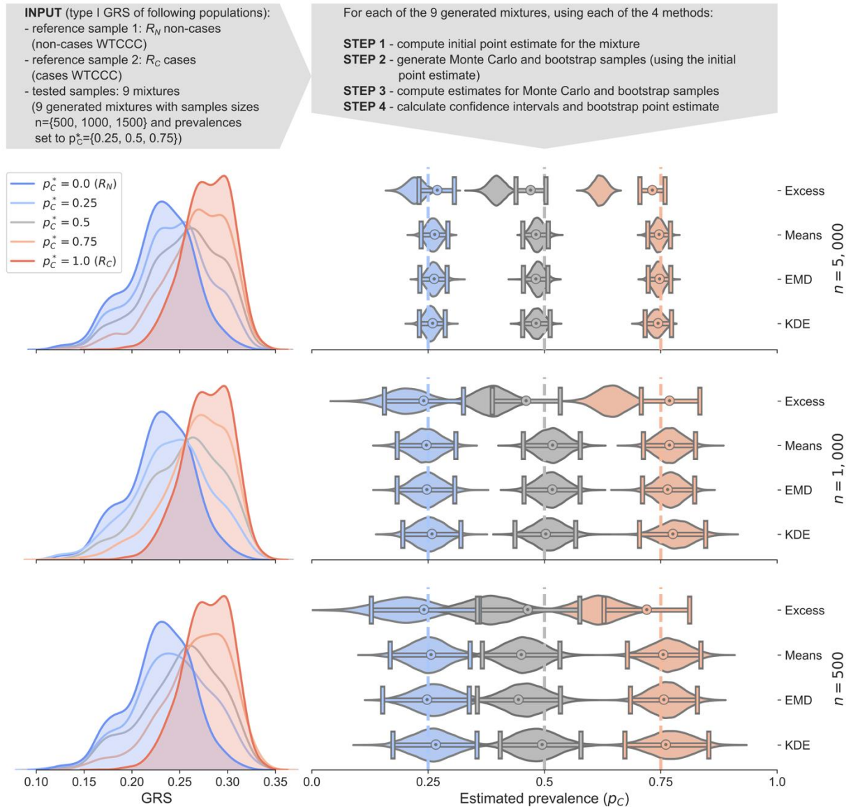
Figure 3: A comparison of the 4 methods prevalence estimates and confidence intervals for varying proportion of disease and for 3 sample sizes. Mixture distributions of controls and Type 1 diabetes patients from WTCCC 6 were constructed with p_C^* = \{0.25, 0.5, 0.75\} (shown in blue, grey and red respectively) and n = \{500, 1000, 5000\} . (Left column) The constructed mixture distributions and reference distributions ( R_C , shaded red and R_N , shaded blue) from which they were constructed. (Right column) Prevalence p_C estimates (bullseye) obtain by each of the 4 methods for varying p_C^* (x-axis) and sample size, n (rows). Each estimated p_C value is shown together with violin plot illustrating the distribution of the 100,000 estimates of prevalence ( p'_C ) in the bootstrap samples and with confidence intervals ( \alpha = 0.05 ; horizontal line with vertical bars at the ends). Dashed vertical lines indicate reference prevalence values p_C^* . In all the cases, for the Excess method we observe a large offset between the violin plots and the p_C value and its confidence interval. This offset is a result of the systematic bias of the Excess method. Employed bootstrap methodology allows
