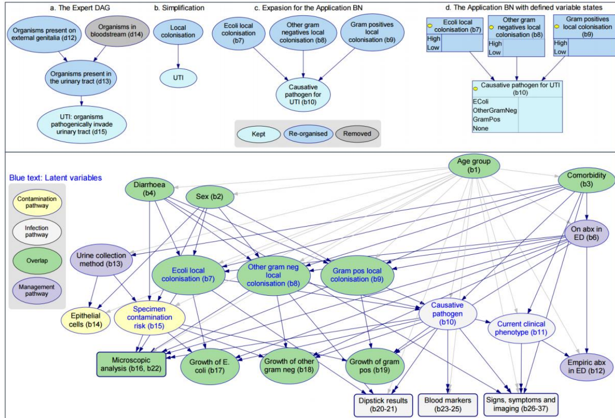
Figure 2. Top: An example of converting from the Expert DAG v11.1 to the Applied BN v2.2. Bottom: The high-level Applied BN structure. Additional file 4 includes a full list of differences between the two models. Additional file 5 presents the detailed structure of the Applied BN, in particular the local structure of submodels microscopic analysis, dipstick results, blood markers, and signs and symptoms (round box in the bottom panel), as well as the BN variable dictionary. The source model file for the Applied BN can be accessed via https://osf.io/8taqy/ .
