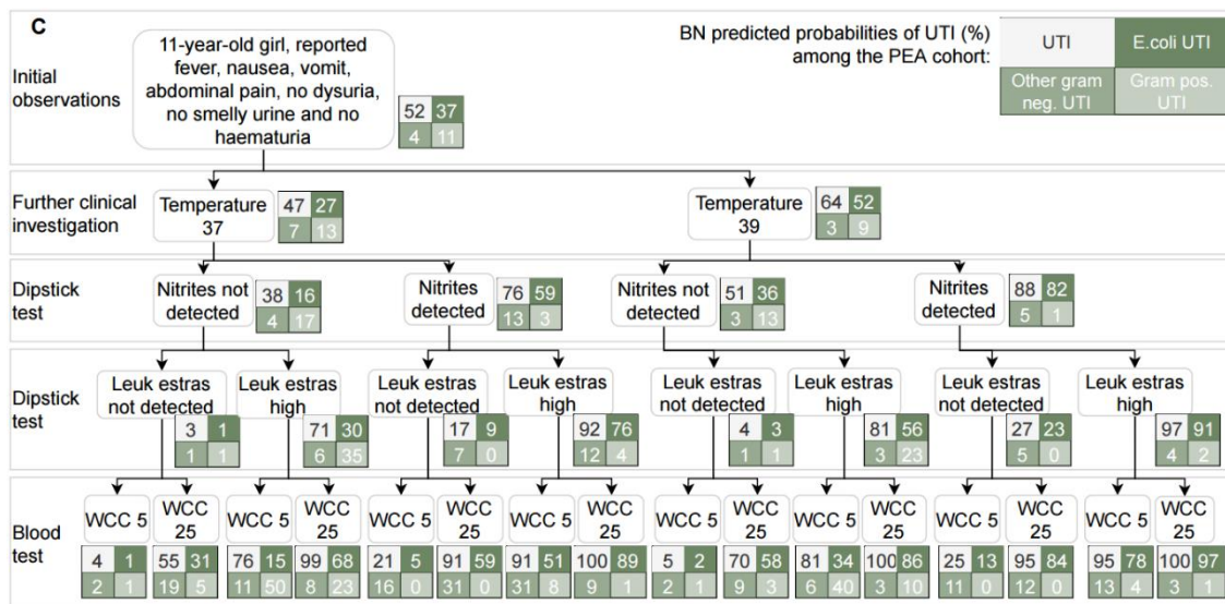
Figure 7. Predictions from the Applied BN under the clinical scenario C.
