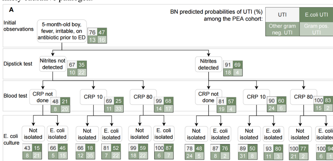
Figure 5. Predictions from the Applied BN under the clinical scenario A.
