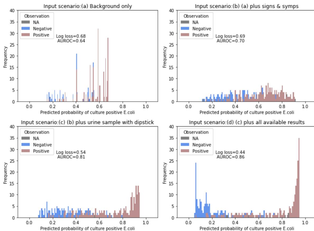
Figure 3. Applied BN v2.2 performance as compared with observations, with Log Loss and AUROC across four scenarios. Each panel presented the distribution of the Applied BN predicted probabilities of
