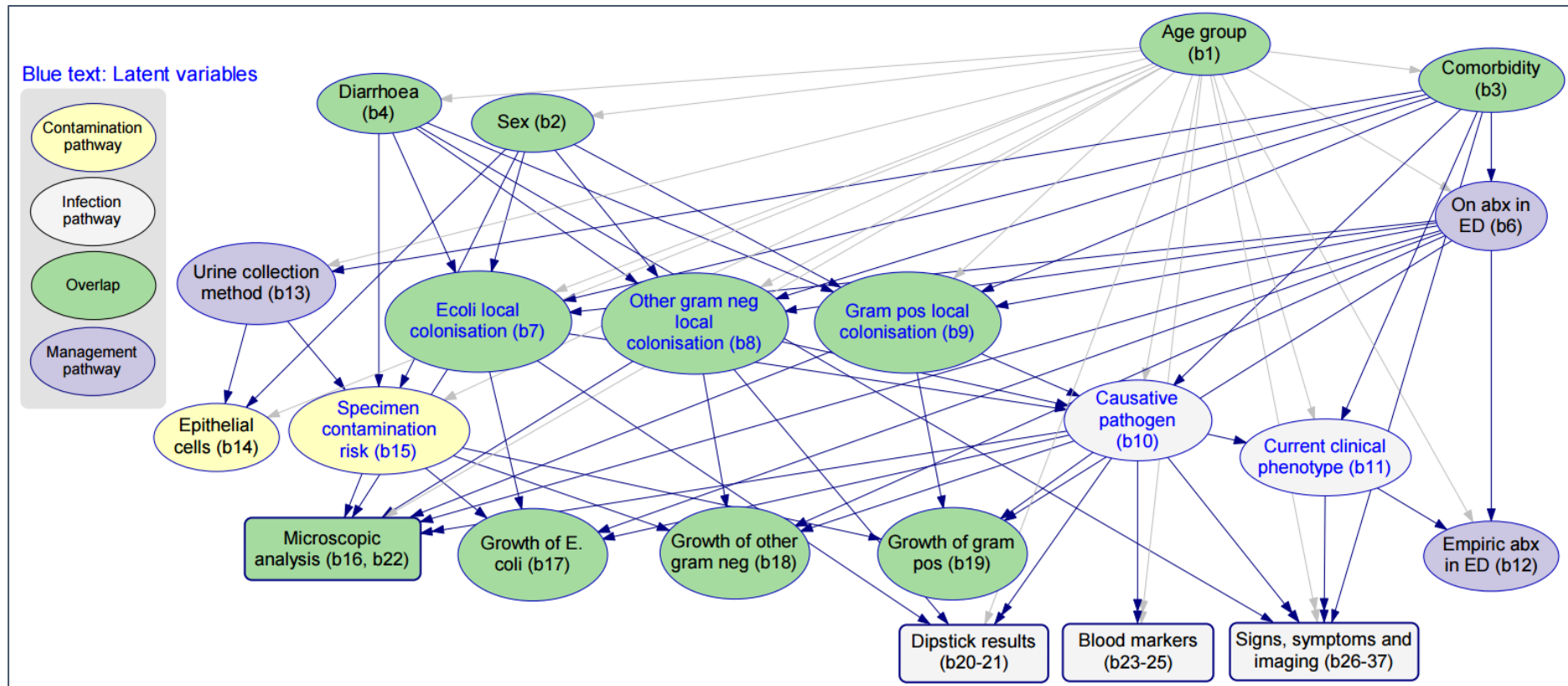
Figure E1. The high-level structure of the Applied BN v2.2, as provided in the main manuscript (Figure 2, bottom panel).
