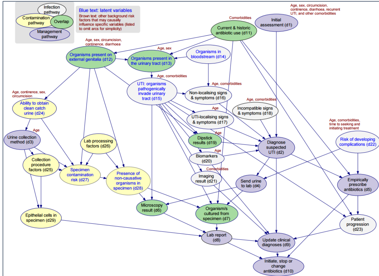
Figure 1. The Expert DAG v11.1. The expert-elicited causal directed acyclic graph describing the relationships between infection (white), specimen contamination (yellow) and UTI management (purple) in children, in particular, variables that fell into more than one pathways were indicated in green. Note: Numbers within the model nodes correspond with the narrative description. A detailed variable dictionary is provided with the supplementary material: Additional file 3. The source model file for the Expert DAG can be accessed via https://osf.io/8taqy/ .
