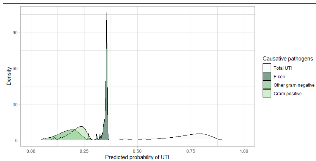
Figure 4. Sensitivity analysis on causative pathogens as the pathogenicity of different organism changes by \pm 20\% .
