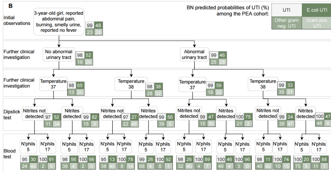
Figure 6. Predictions from the Applied BN under the clinical scenario B.
