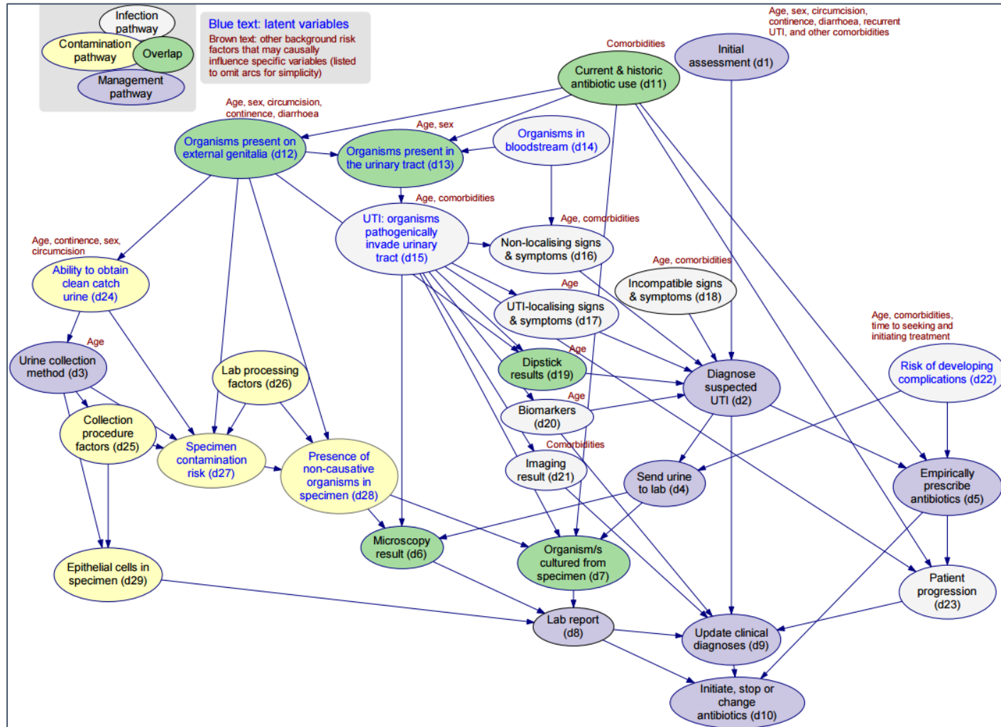
Figure C1. The Expert DAG v11.1, as provided in the main manuscript (Figure 1).
