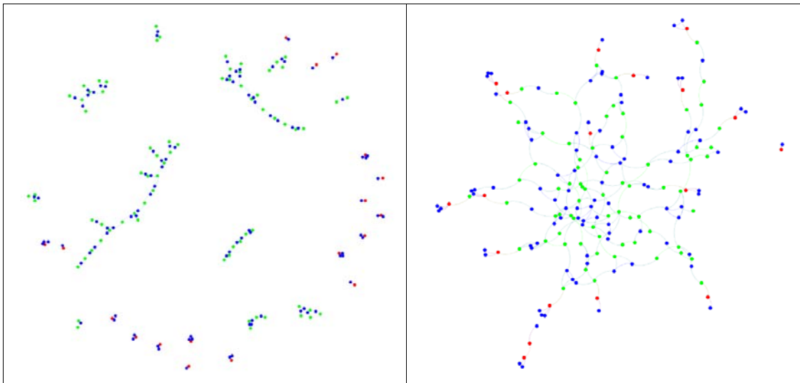
208 Figure 1: Plots of ‘toy’ contact networks (representing a reduced number of nodes for visual 209 illustration of N=186) with different levels of DSPHs and Bubbling. (Top-left) Baseline model without 210 any discordant-parentage and without any bubbling, (Top-right) bubbling only. (Bottom-left) 211 discordant-parentage only, and (Bottom-right) both discordant-parentage and bubbling. Nodes are 212 colour code as follow: Blue dots – children, Green dots – parents in households where both parents 213 retain contact with offspring, and Red dots – parents who are the sole parent having regular contact 214 with their offspring.
