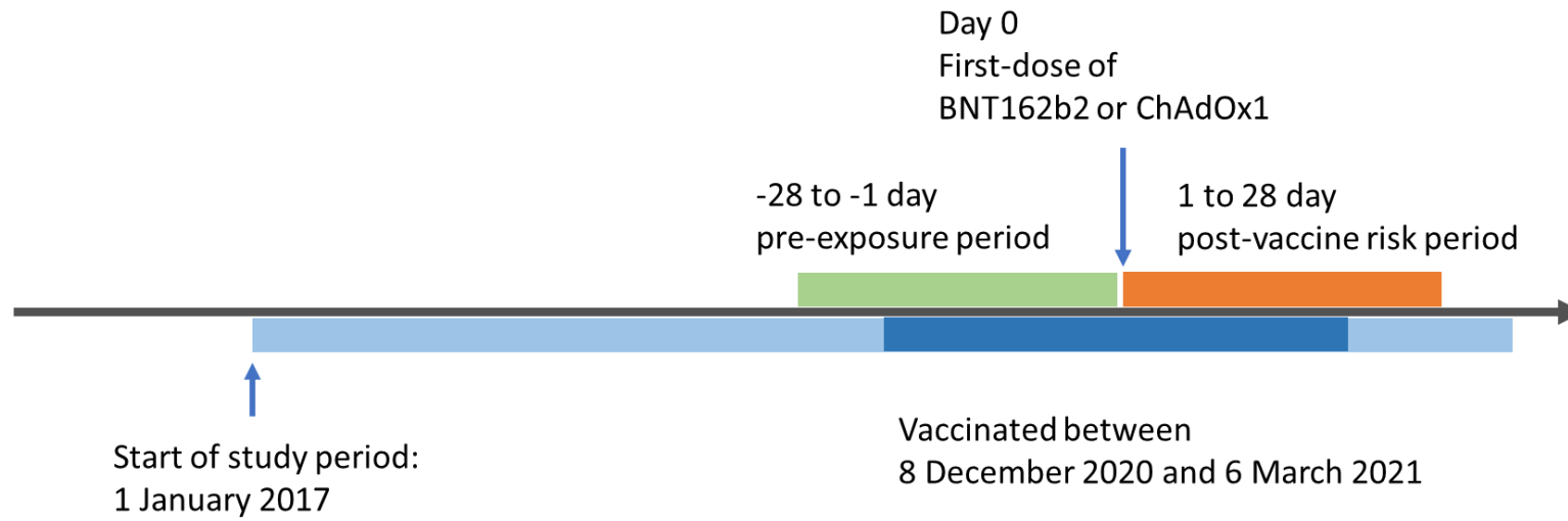
Figure 1. Self-controlled case series analysis design
