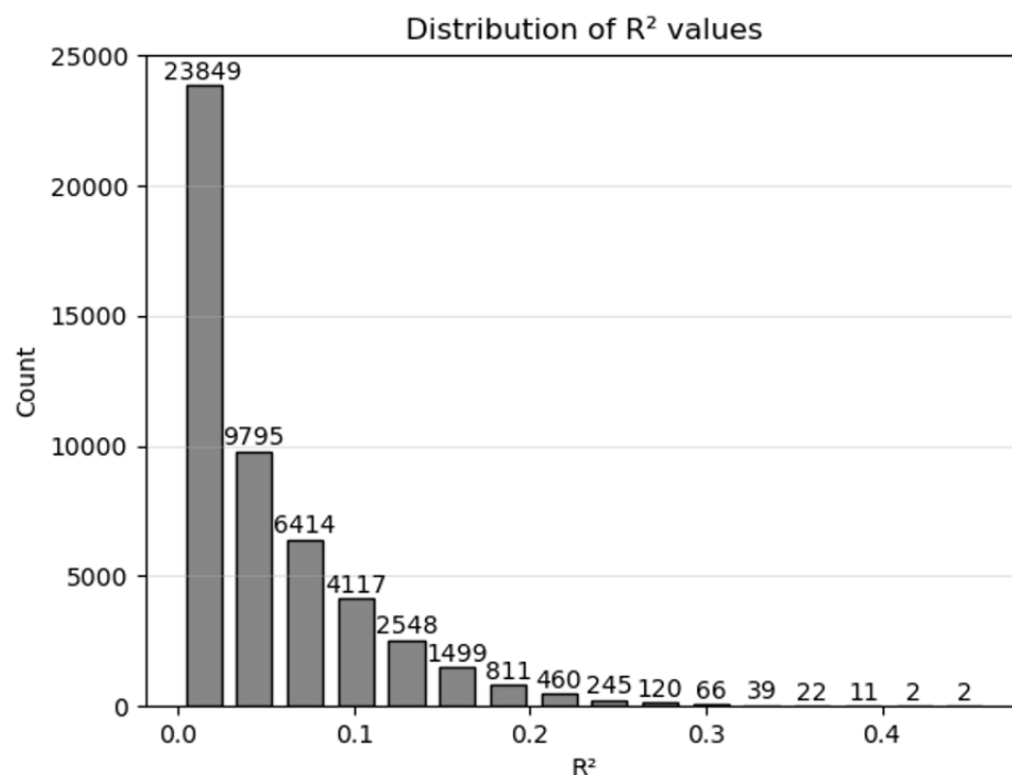
Figure 2. Distribution of R^2 values from 50,000 random samples. The graph above demonstrates the degree to which R^2 = 0.493 may be considered an outlier. Of 50,000 random samples of the full dataset, the most extreme R^2 observed was 0.461, indicating that such a result as reported by Miller and Goldman is statistically improbable.
