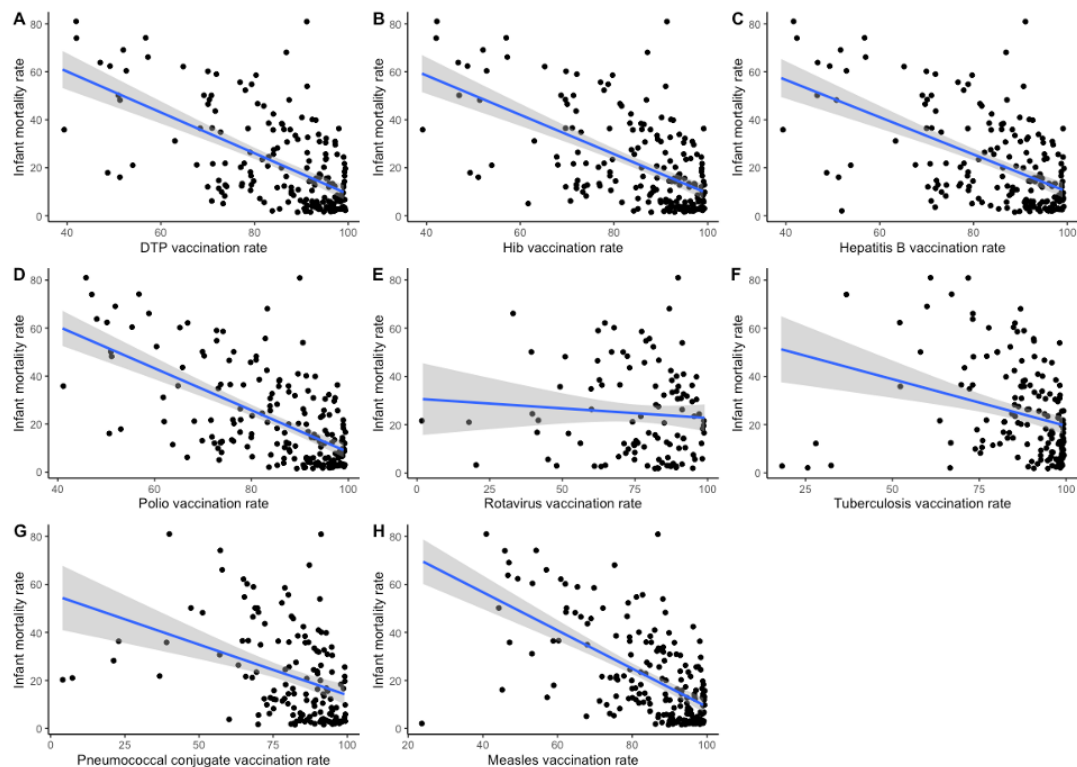
Figure 3 - Vaccination rate and infant mortality. For 8 vaccines with global vaccination rate data, we plotted the association with each nation's infant mortality rate. We also calculated the linear regression statistic for each data set: DPT vaccine correlation coefficient = -0.85 and p-value = 4.19E-21, Hib vaccine correlation coefficient = -0.81 and p-value = 1.45E-19, HepB vaccine correlation coefficient = -0.77 and p-value = 2.62E-17, Polio vaccine correlation coefficient = -0.87 and p-value = 4.76E-22, Rotavirus vaccine correlation coefficient = -0.079 and p-value = 0.41, Tuberculosis vaccine correlation coefficient = -0.38 and p-value = 1.04E-04, PCV vaccine correlation coefficient = -0.42 and p-value = 2.29E-06, Measles vaccine correlation coefficient = -0.79 and p-value = 4.93E-21.
