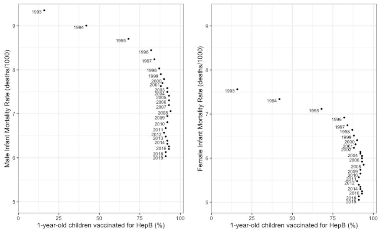
Figure 4: Hepatitis B Vaccine Administration Compared to Male and Female IMR in the United States by Year. These graphs demonstrate a moderate negative correlation between percent of children vaccinated for Hepatitis B and IMR for both males and females in the United States (Spearman Correlation Coefficient = -.665 , p -value = .000152 ).
