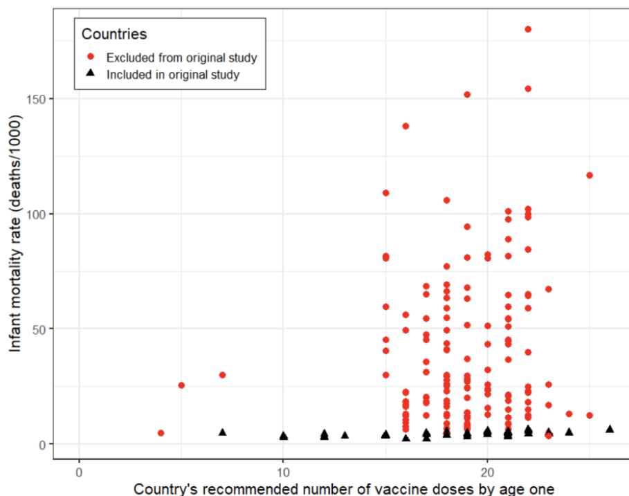
Figure 1: 2009 Vaccine Dose and IMR Data Exclusion. The graph above shows a stark contrast between the data used in Miller and Goldman’s study (in black), and the data in the dataset that was available for that study (in red). Using only a very small subset of the available data, the original study showed a moderate correlation between the number of scheduled vaccine doses and IMR ( R^2 = 0.493 ). However, when the full dataset is included, the correlation is near zero ( R^2 = 0.026 ), indicating that these two variables are unrelated. Thus, the exclusion of data dramatically changed the conclusion of the data analysis.
