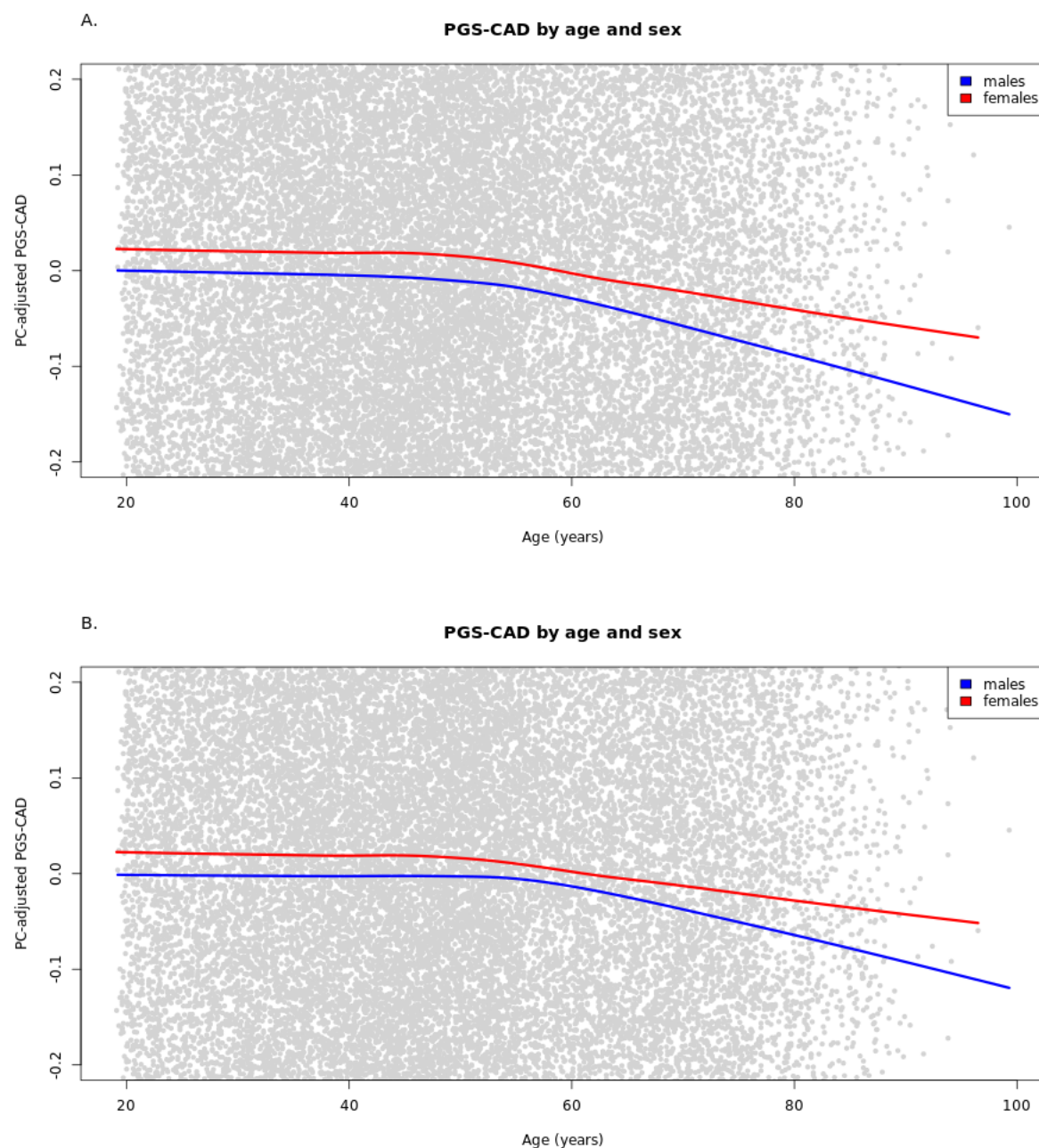
Figure 1. Raw PGS CAD by age and sex in the cohort baseline. Illustration of the selection bias in the cohort baseline using lowess curves for PGS CAD by age for males and females separately. The plot has been zoomed in relative to the y-axis to better show the trends. Panel A shows the trends in the analysis dataset used in the Cox models (prevalent cases excluded) and panel B when prevalent cases are included.
