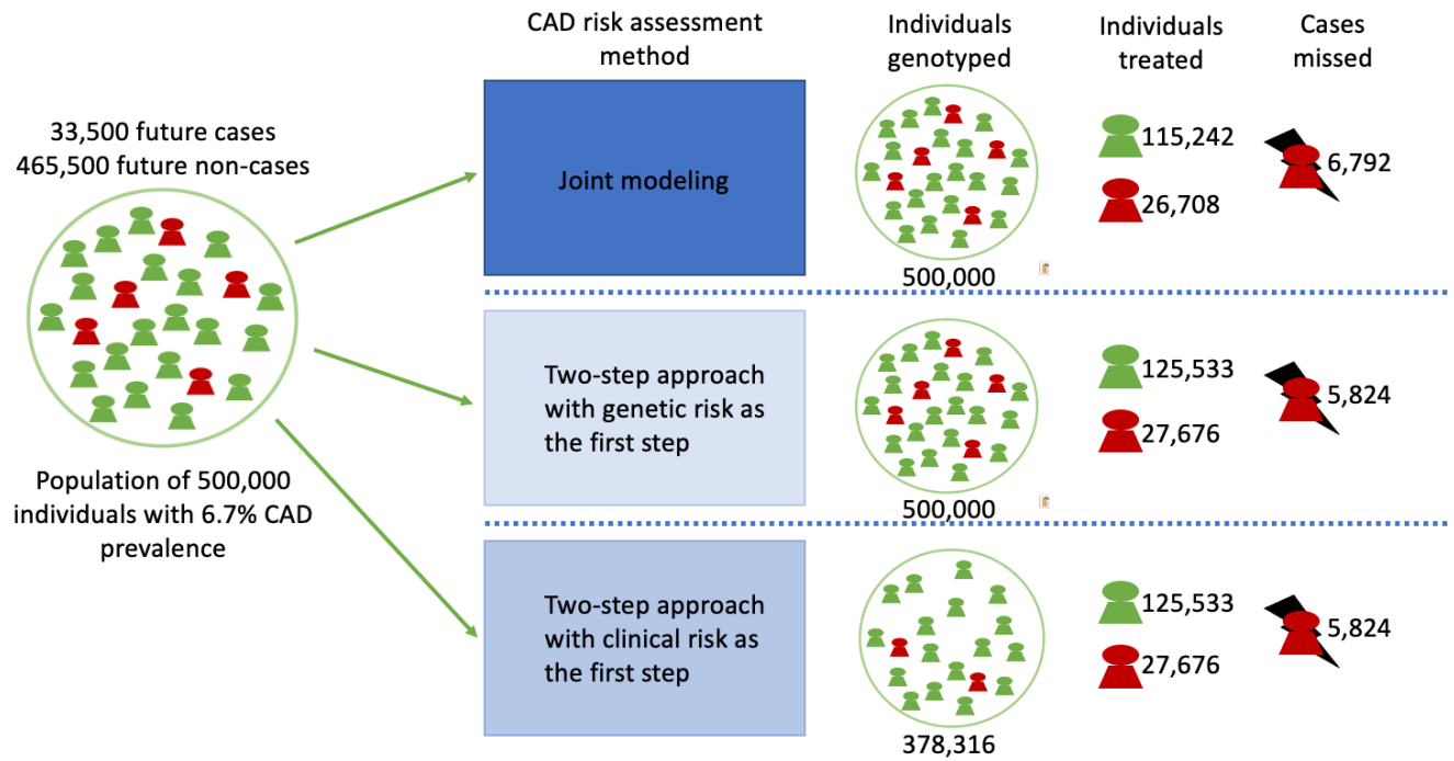
Figure 4. Demonstration of the different risk models implementing clinical and genetic risk with interactions in a hypothetical population of 500,000 people. The CAD prevalence used in the demonstration is based on the current CAD prevalence in the US.
