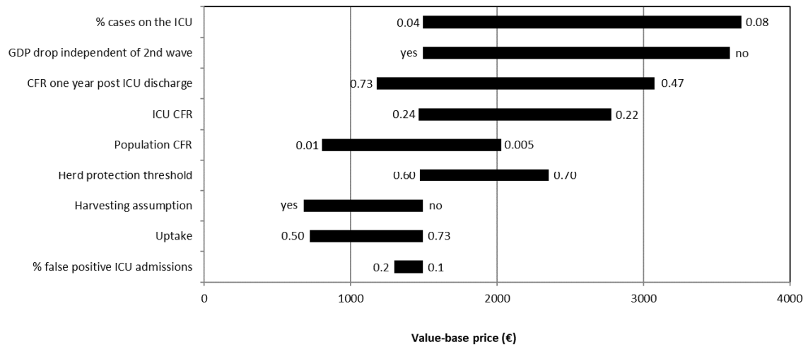
Figure 1. Tornado diagram demonstrating the results of the one-way sensitivity analysis. The variables are ordered by the impact on the value-based price of a COVID-19 vaccine based on an absolute rule (95% efficacy). The numbers indicate the upper and lower bounds.
