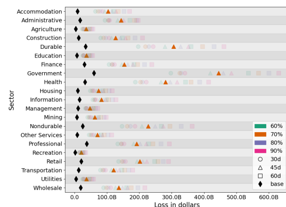
Figure 8: Sector level total loss for each scenario. The black and orange markers are highlighted to show the unmitigated and mitigated case VHI_70_SH_70_45 respectively. Percentages are compliance to NPIs and “d” is the duration of SH order.
