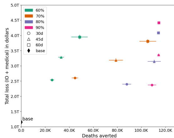
Figure 6: Trade-off between the number of deaths averted and economic losses under each scenario. The vertical and horizontal bars show the inter-quartile range.
