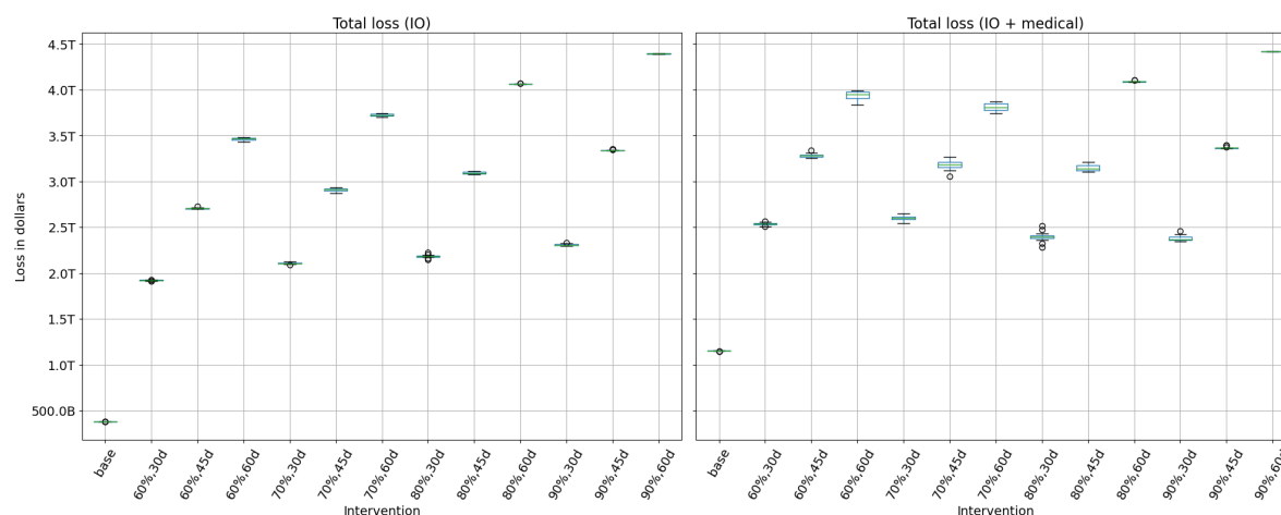
Figure 4: The left subfigure shows I-O economic losses (without medical costs) due to NPI measures and infections for each of the scenarios. The percentages show compliance to NPIs and “d” is for the duration of the Stay-home order. These losses arise from the drop in labor supply to sectors, caused by lockdown, illness and mortality, and from interdependencies between sectors. It does not include the economic burden imposed by the treatment and medical services provided to the infected individuals, whereas the right subfigure includes this medical burden.
