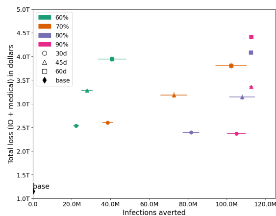
Figure 5: Trade-off between the number of infections averted and economic losses under each scenario. The vertical and horizontal bars show the inter-quartile range.
