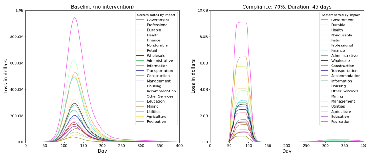
Figure 9: Sector level daily losses caused by the inoperability of each sector and its cascading impact on other sectors due to interdependencies between sectors. The left subfigure shows losses for the unmitigated case. The right subfigure shows losses for the mitigated scenario VHI_70.SH_70.45. The ordering of sectors in the legend is ranked by the height of the curve. Note that the scale of loss (y-axis) in the right subfigure is ten times of the left subfigure.
