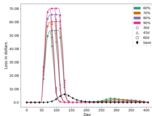
Figure 7: Daily I-O loss across all sectors for each scenario. The unmitigated base case is shown by the black curve where no NPIs are in place. Percentages are compliance to NPIs and “d” is the duration of SH order.
