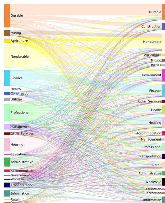
Figure 3: This figure shows interdependencies between sectors as given by the US Bureau of Economic Analysis. The left sector flows are input to right sectors.
