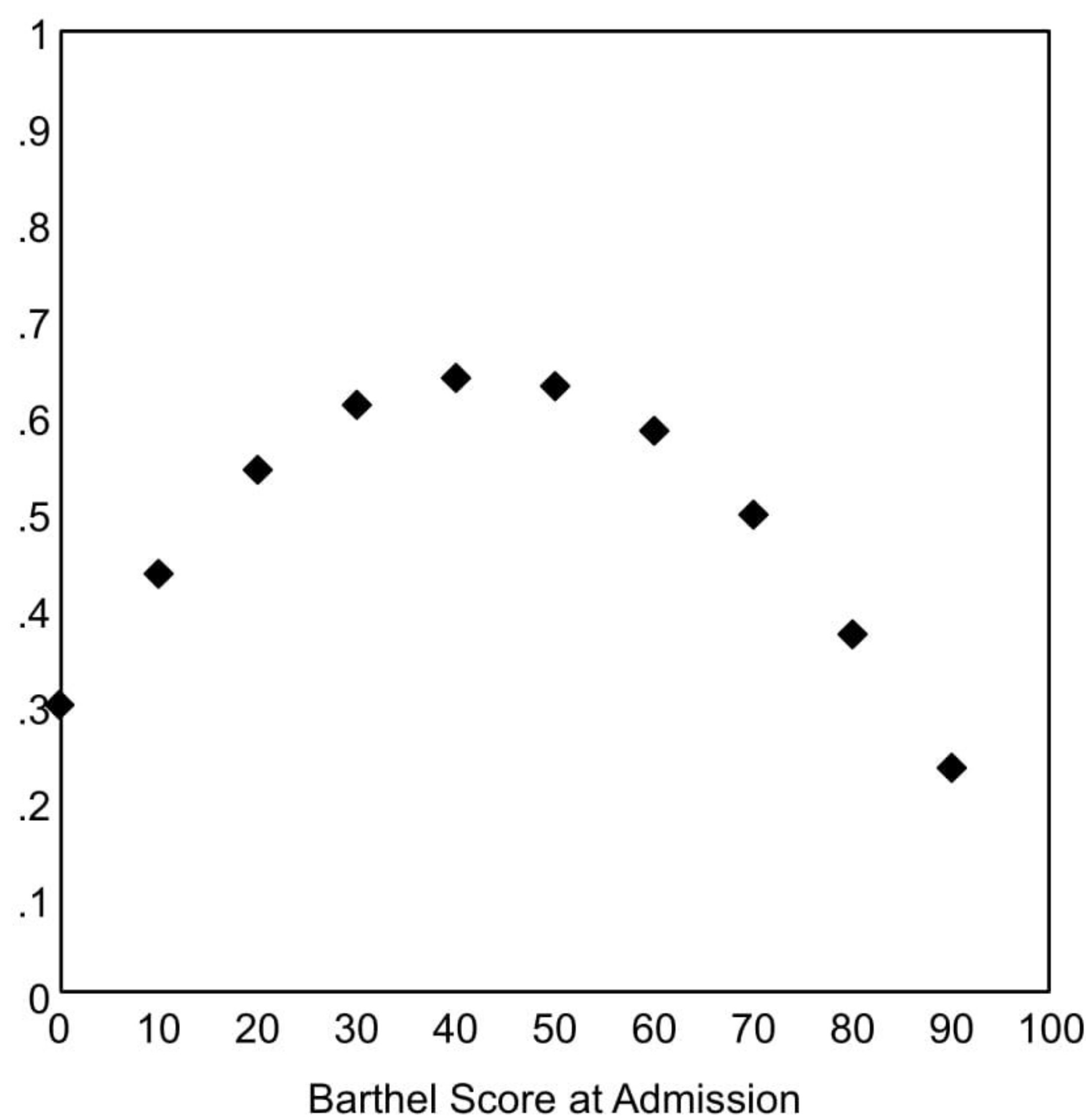
Figure S1. Results from Bayesian multilevel logistic regression models for Barthel improvement \geq 10 points: predicted probability of improvement as a function of Barthel score on admission. Emilia-Romagna, year 2017.
