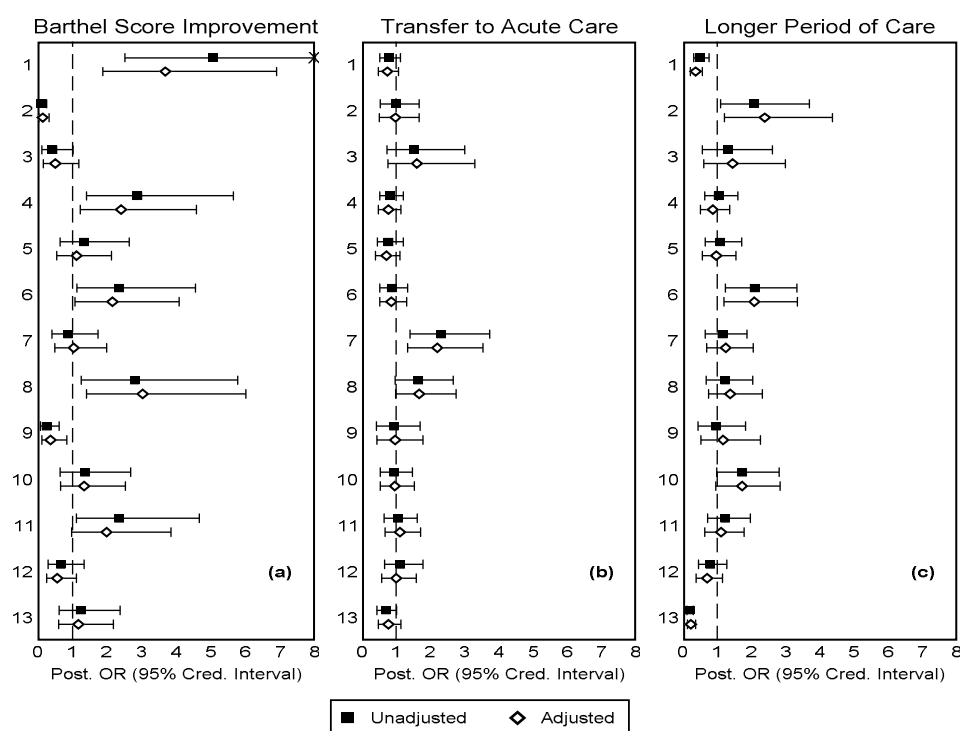
Figure 1. Results from Bayesian multilevel logistic regression models for (a) Barthel improvement \geq 10 points, (b) transfer to acute care hospital, and (c) length of stay \geq 20 days: hospital-specific odds ratios (ORs), unadjusted and adjusted for patient case mix, Emilia-Romagna, year 2017. Dashed line indicates the null value of 1 (no difference compared to the overall average).
