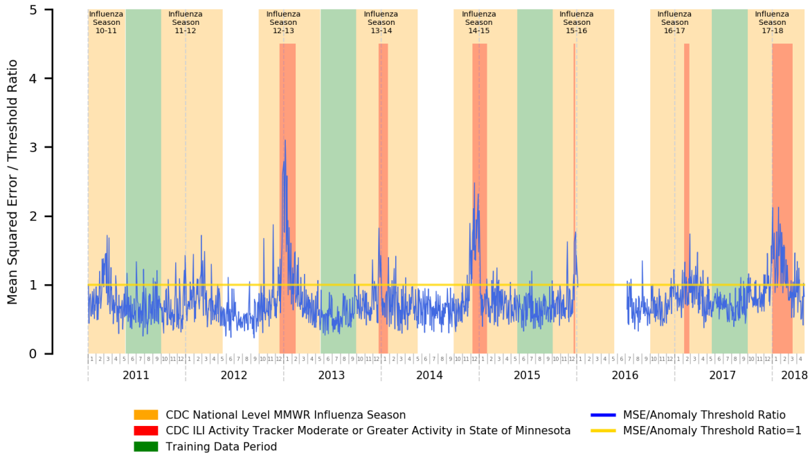
Figure 1 - Mean Squared Error Relative to Anomaly Threshold for an Autoencoder Trained for the Influenza Season Detection Task
