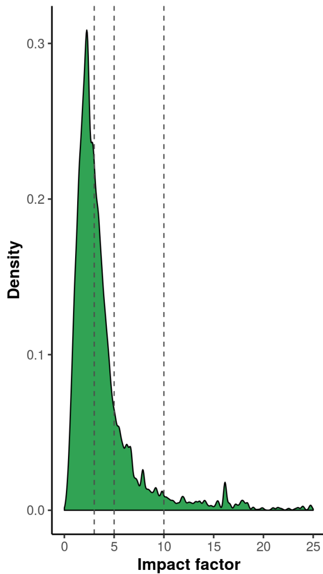
Supplementary Figure S1. Distribution of journal impact factors (JIFs) of analyzed RCTs with JIF cutoffs of 3, 5 and 10 (dotted lines). The JIF of a journal in the year following the publication data of the RCT was used. Density represents the probability of a trial to belong to a given impact factor.
