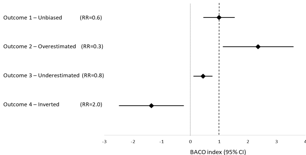
Fig. 2 BACO indices of four simulated composite outcomes.
