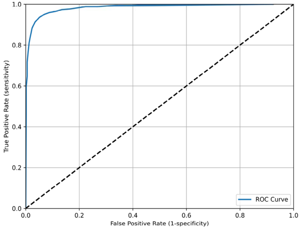
Figure 4. Receiver operating characteristics curve of the algorithm for hold-out test data predictions up to six hours before sepsis onset.
